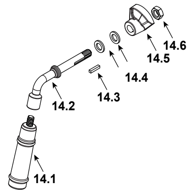
#14 Door Handle Assembly
