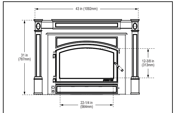
Figure 3.5 - Front View with Small Flat Surround (CT2-4331) with Cast Trim (811-0930)
