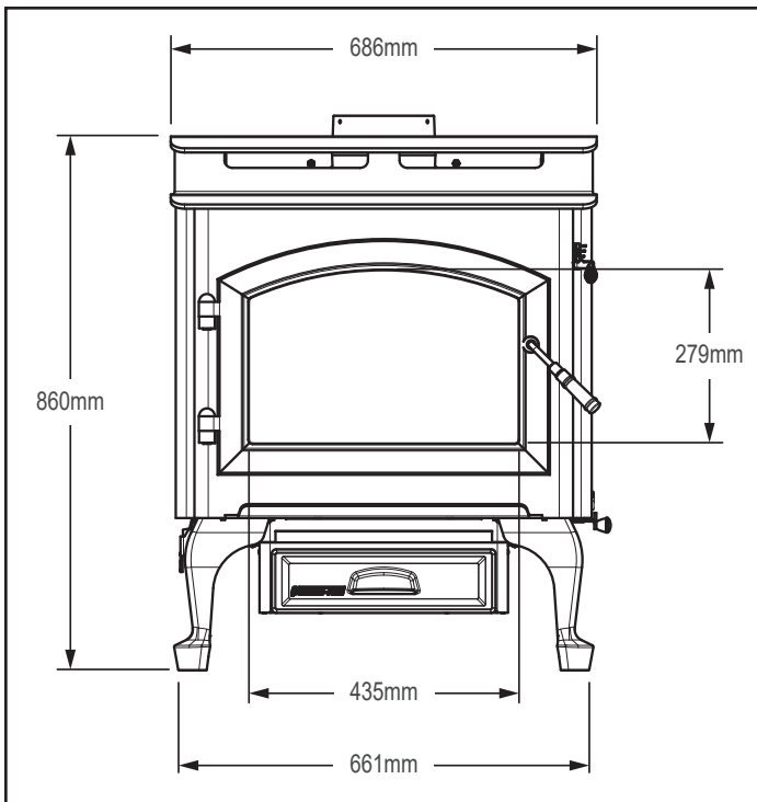
Figure 8.1 - Front View
