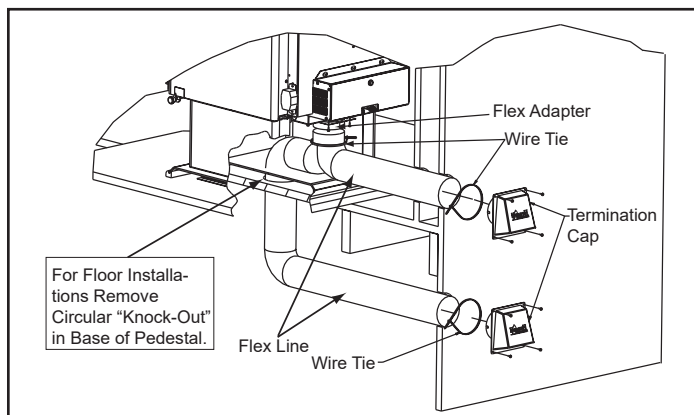
Figure 20.1 - Floor & Rear Installation
