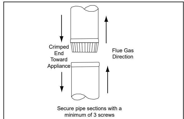
Figure 13.1 - Chimney Connector (Appliance Pipe)
