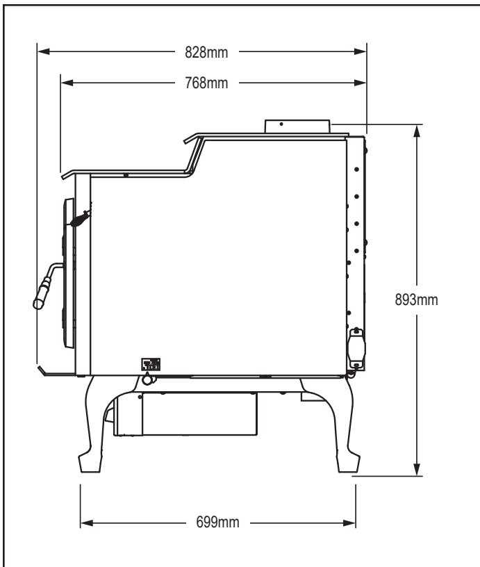
Figure 8.2 - Side View
