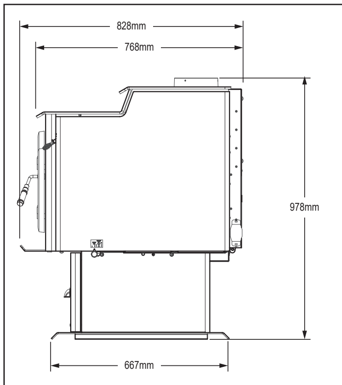
Figure 7.2 - Side View
