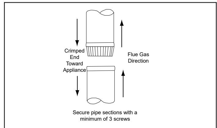
Figure 13.1 - Chimney Connector (Appliance Pipe)
