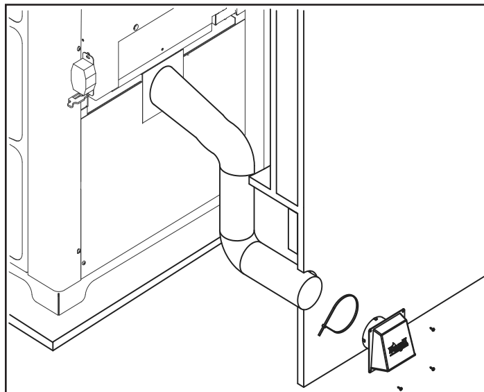
Figure 16.2 - Floor Installation
