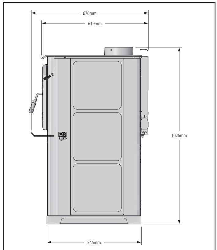
Figure 7.3 - Side View
