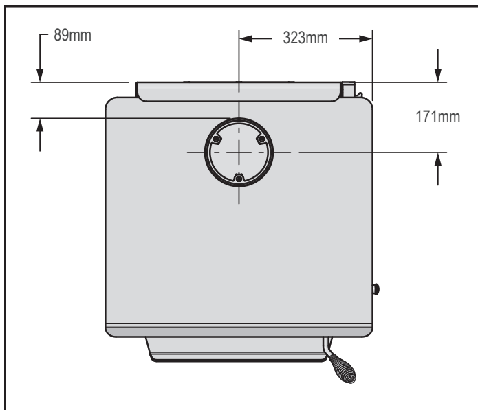
Figure 7.2 - Top View
