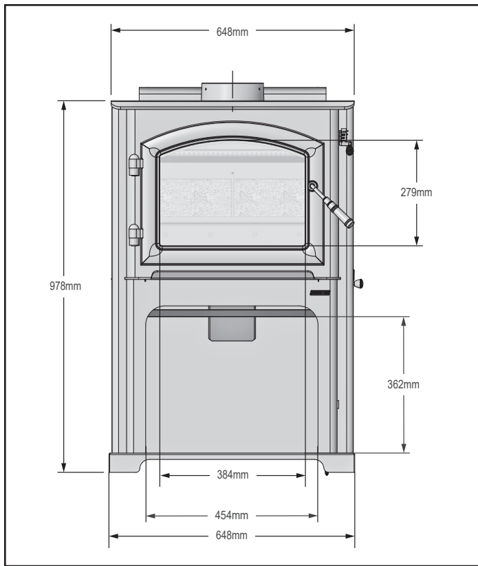
Figure 7.1 - Front View
