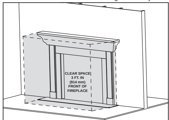
Figure 3.1 Clear Space Requirement - All Models
