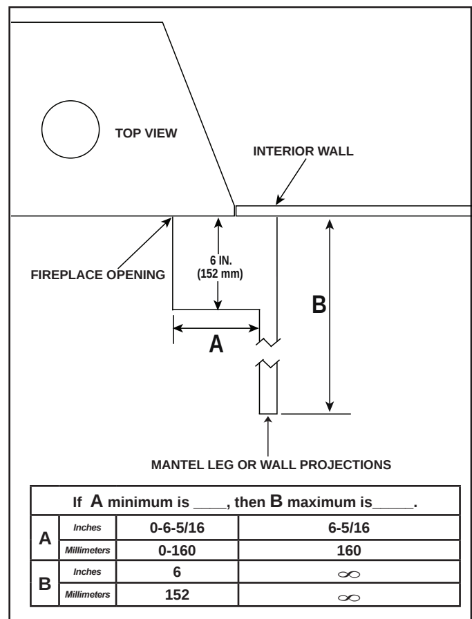
Figure 10.9 Non-Combustible Mantel Leg or Wall Projections (Acceptable on both sides of opening)
