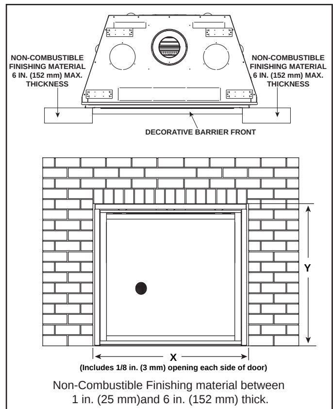
Figure 10.11 Inside Fit Decorative Barrier Front
