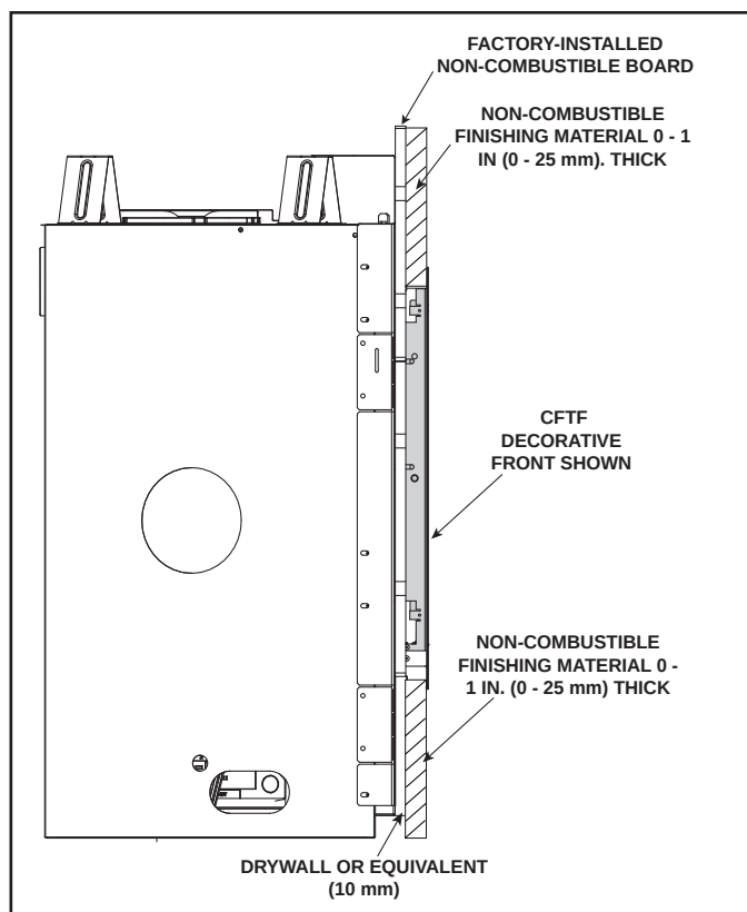
Figure 10.8 Overlap Fit Method (CFTF Decorative Front)
