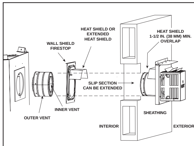
Figure 7.13 Venting Through the Wall
