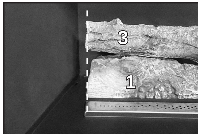
Figure 6 Log #1 and Log #3 Alignment
