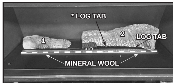
Figure 4 Place Log #2 - Mineral Wool Placement
