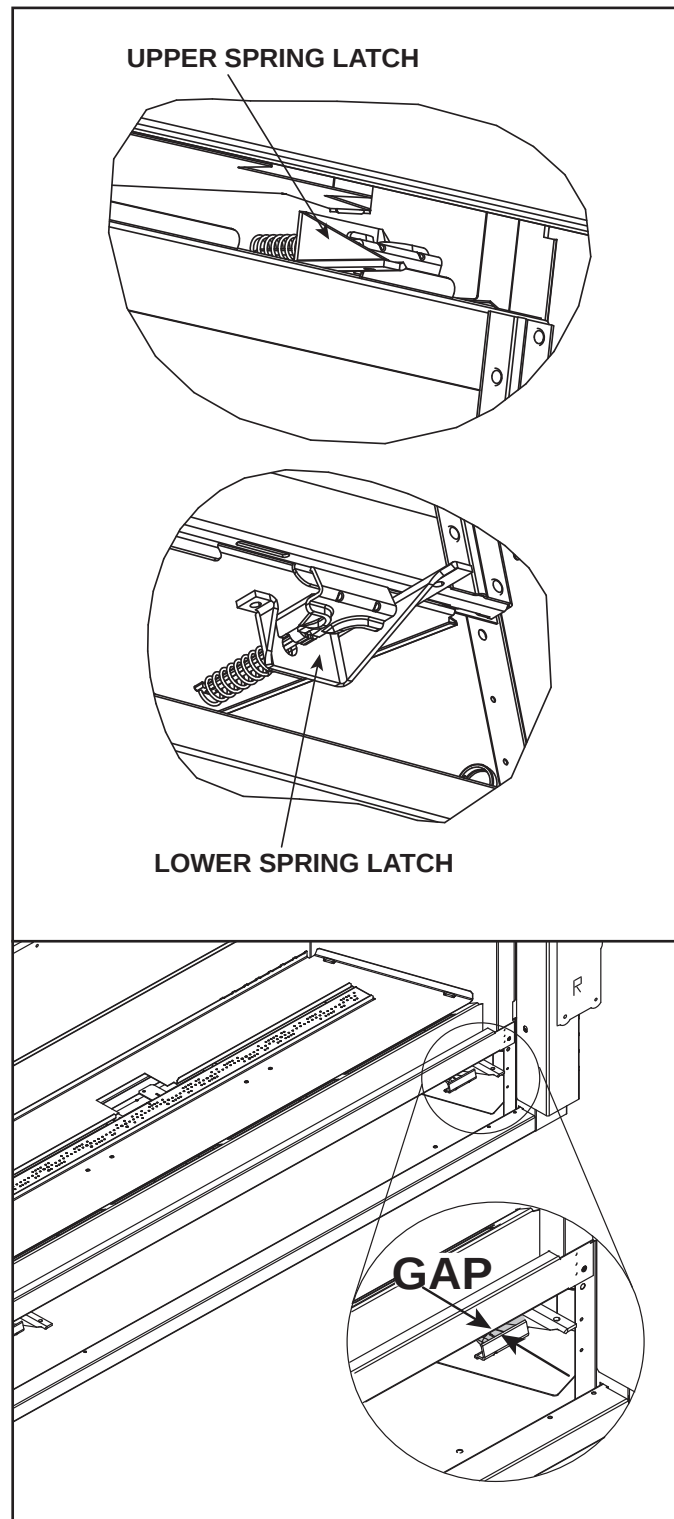
Figure 11.1 Fixed Glass Assembly
