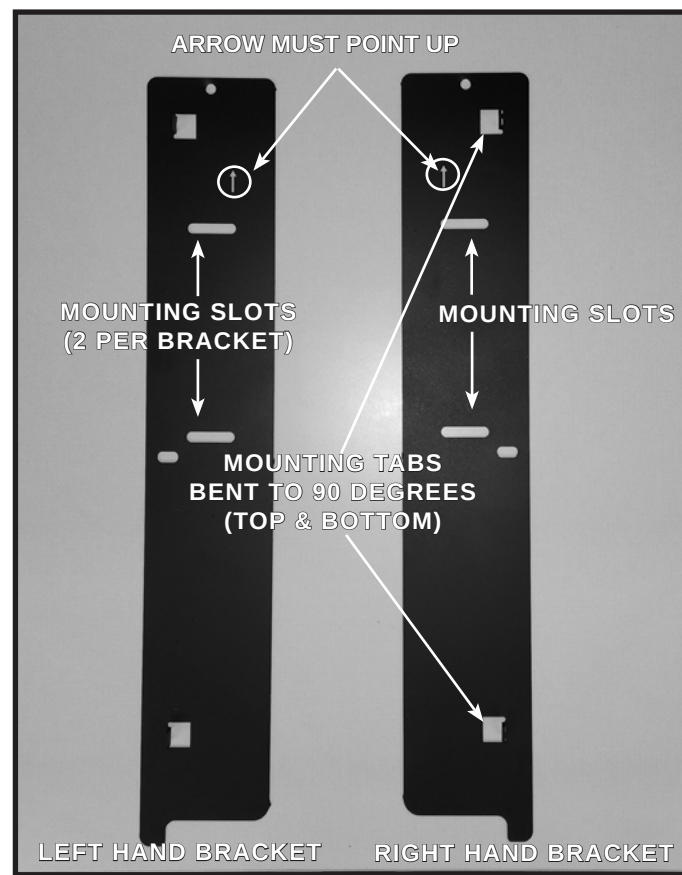
Figure 6.6 Auxiliary Hanging Brackets - Bent For Installation
