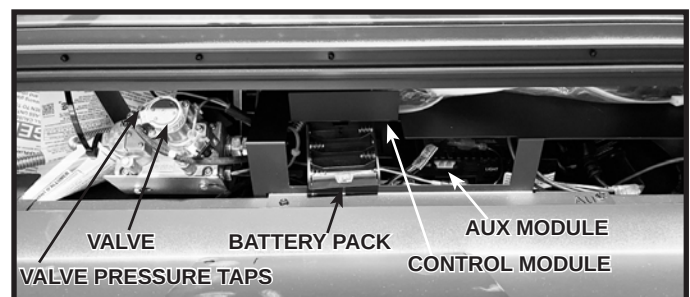
Figure 8.2 Gas Valve, Battery Pack, Control Module & AUX Module
