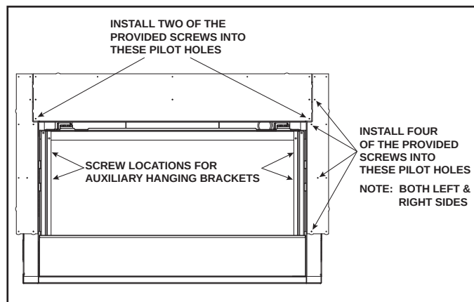
Figure 6.5 Installation of the Side Non-Combustible Components
