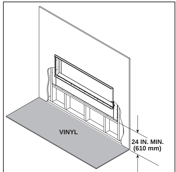
Figure 3.5 Vinyl Flooring Recommendations
