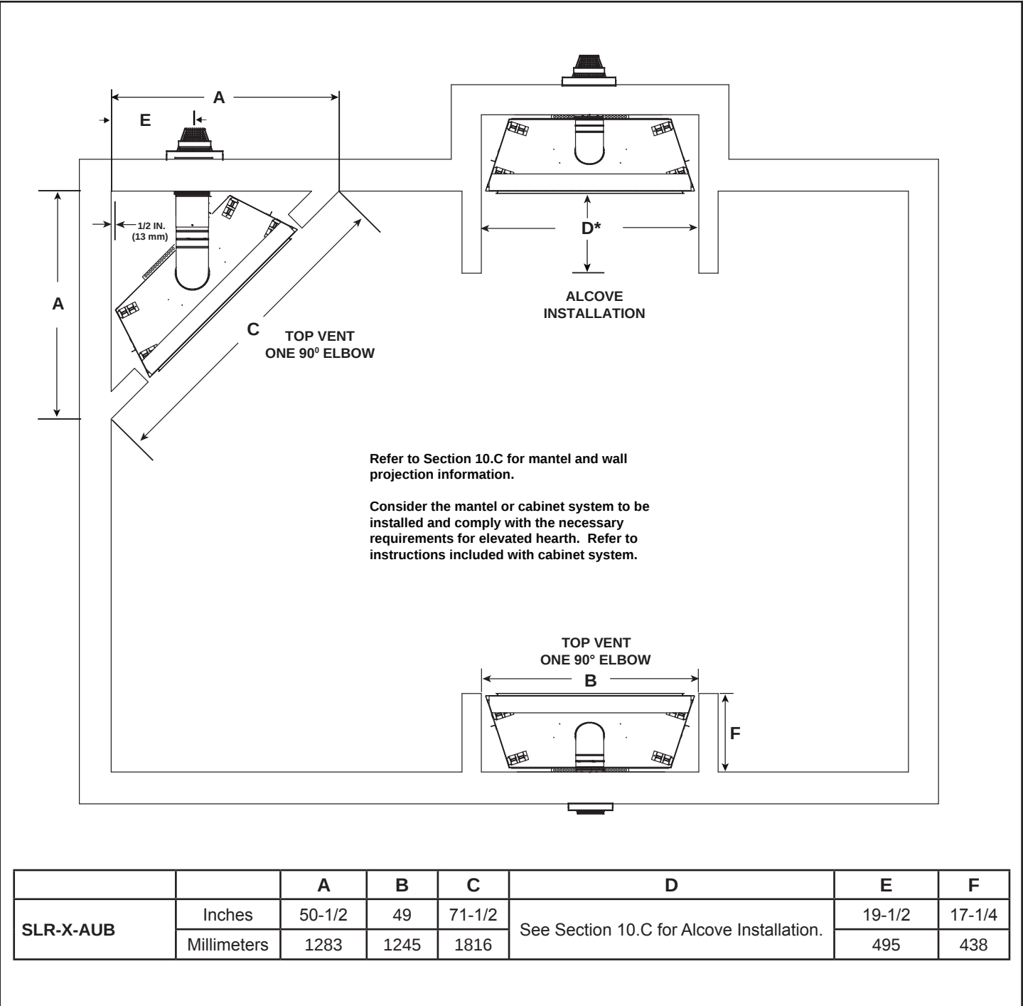
Figure 3.3 Appliance Locations
