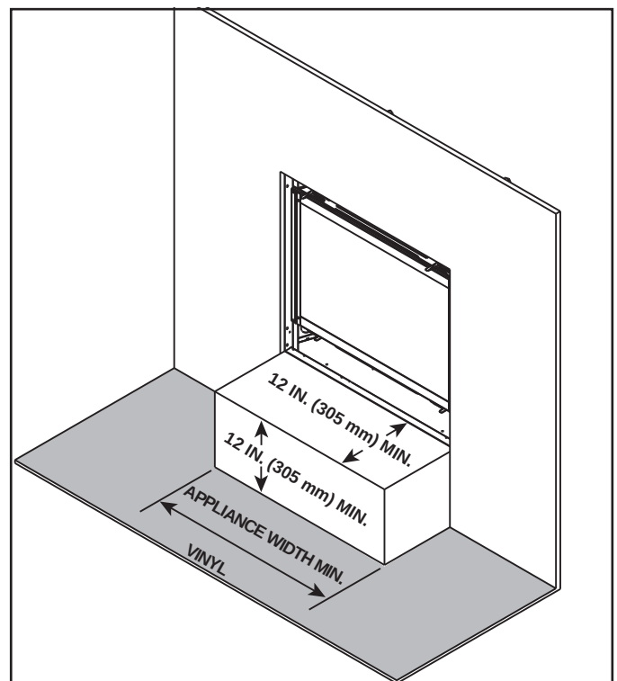
Figure 3.6 Vinyl Flooring Recommendations
