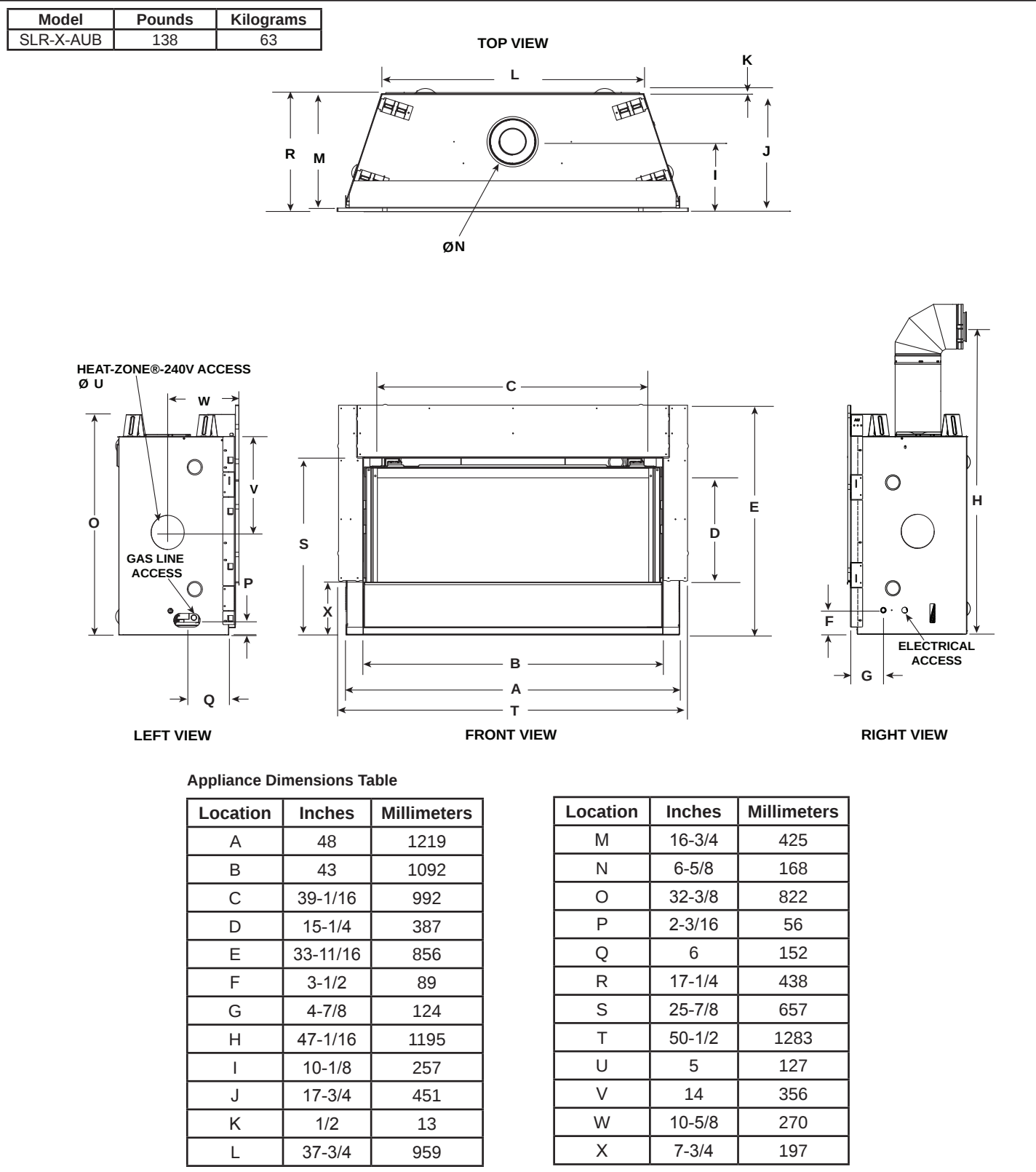
Figure 3.1 Appliance Dimensions
