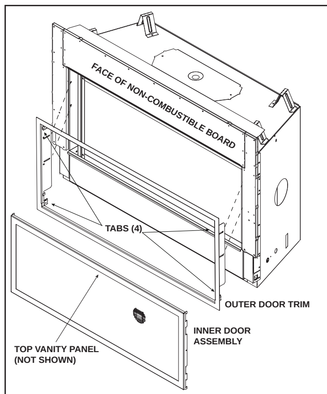
Figure 10.9 CFTF Front Installation With Outer Door Trim
