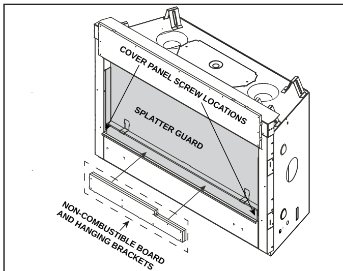
Figure 6.4 Shipping Position - Non-Combustible Sides and Auxiliary Hanging Brackets
