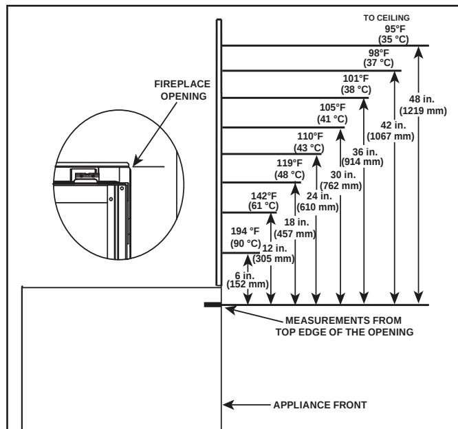
Figure 2.1 Good Faith Wall Surface Temperatures Above Appliance
