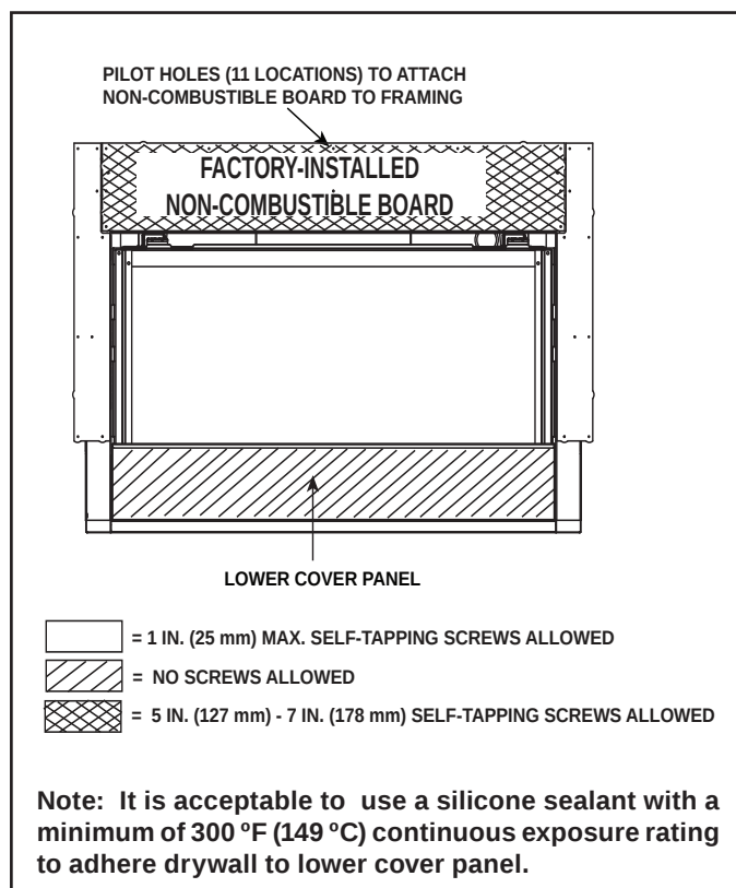
Figure 10.2 Finishing Details
