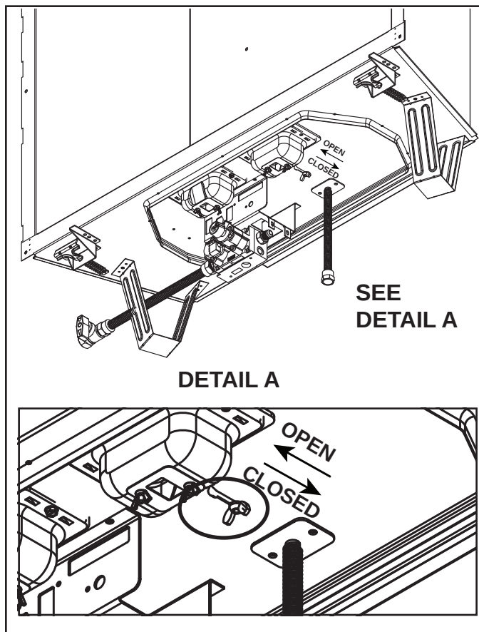
Figure 9.1 Air Shutter Adjustment
