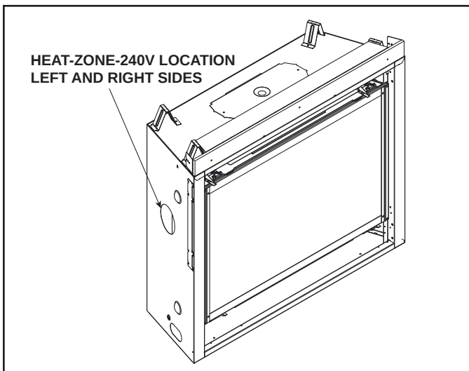
Figure 6.13 Heat-Zone-240V Locations
