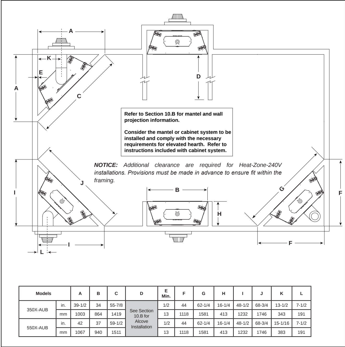
Figure 3.3 Appliance Locations
