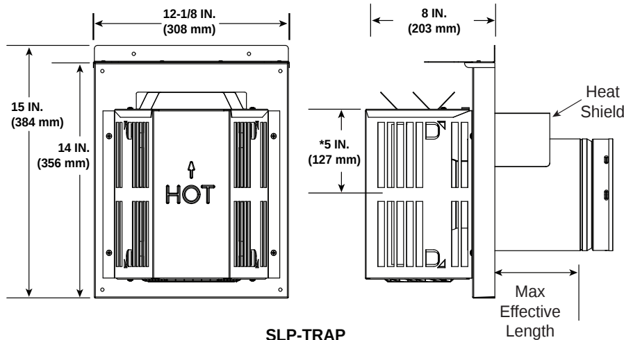
SLP-TRAP Horizontal Termination Cap
