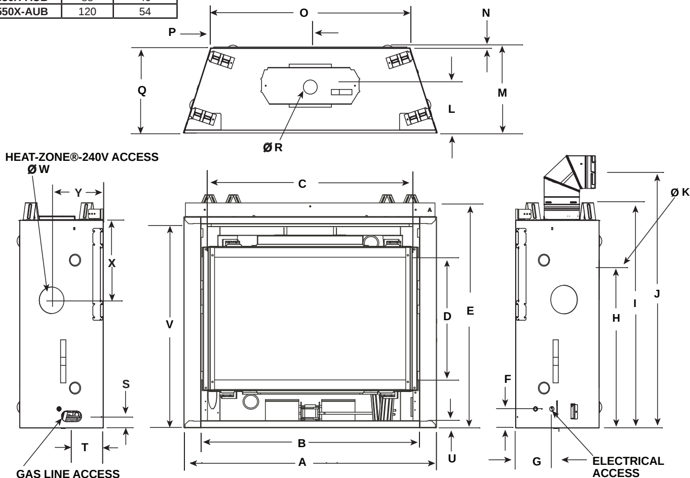
Appliance Dimensions Table
