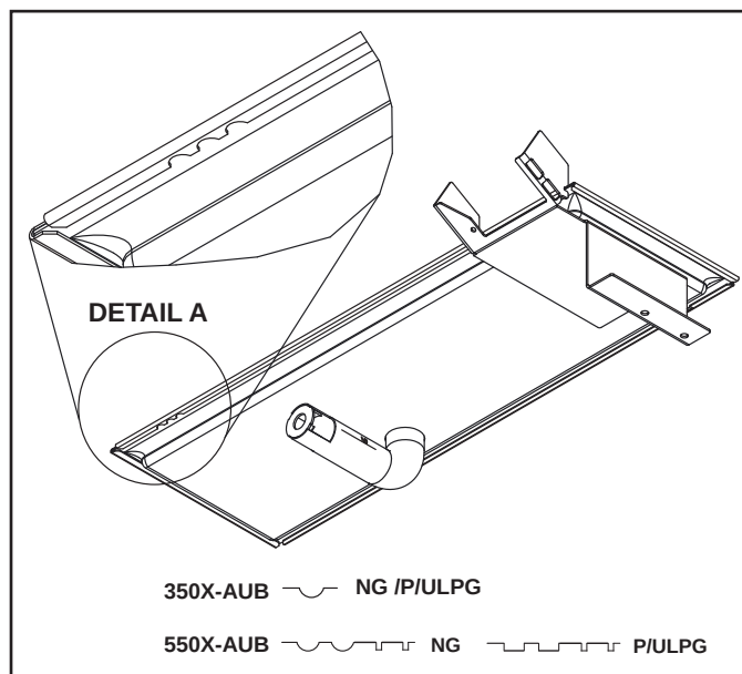
Figure 9.2 Burner Identification
