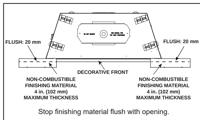
Figure 10.8 Firescreen Decorative Barrier Front
