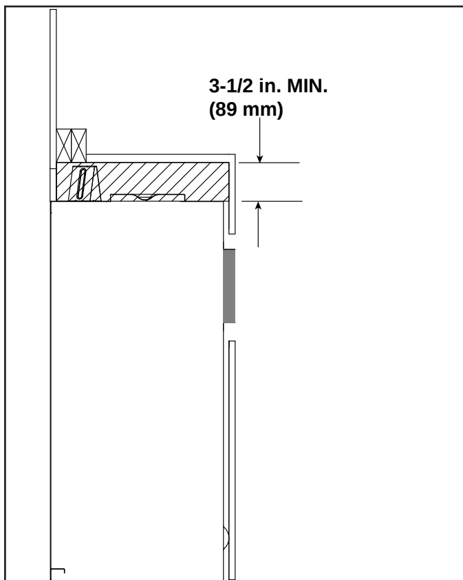
Figure 10.6 Non-Combustible Zone Above Appliance
