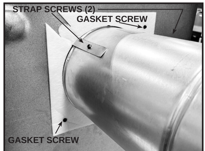
Figure 6.12 Attach the first vent section (it will snap into place). Slide the insulation gasket onto the vent section, up against the appliance. Use two self-tapping screws to secure the corners opposite the gasket tabs. Secure the first section of venting to the fireplace by screwing through the two strap ends left over from cutting the seal cap strap.
