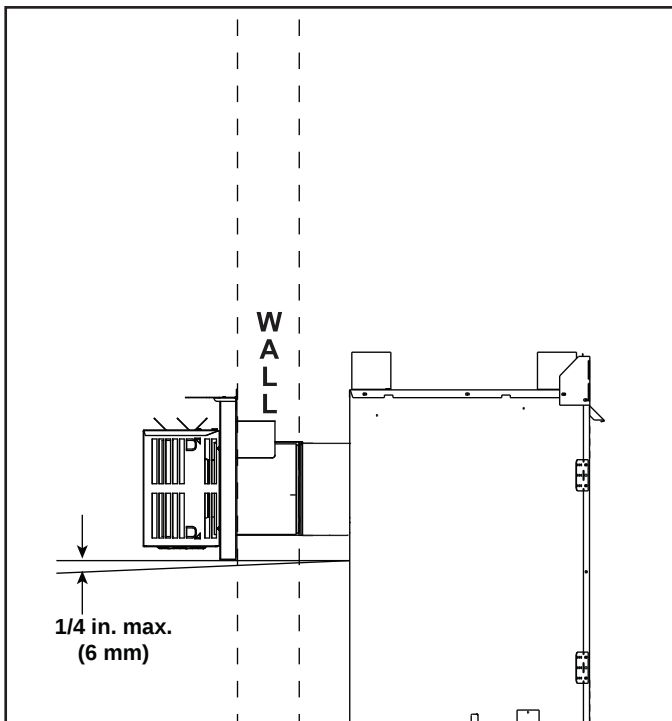
Figure 4.8 Vent Cap - Generic Appliance Shown
