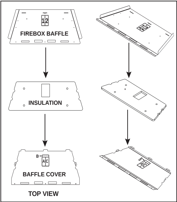
Figure 5.3 Firebox Baffle System
