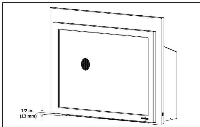
Figure 8.4 Minimum Required 1/2 in. (13 mm) Gap to Bottom of Front
