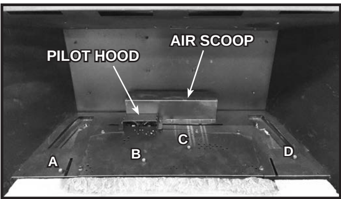
Figure 2. Empty Firebox with Front Hearth Installed
