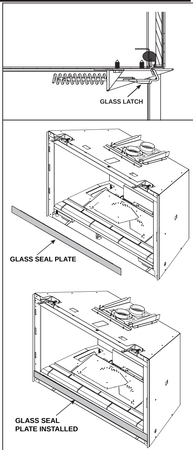
Figure 9.2 Glass Seal Plate and Glass Latch
