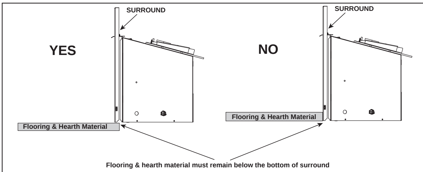
Figure 8.8 Flooring & Hearth Material
