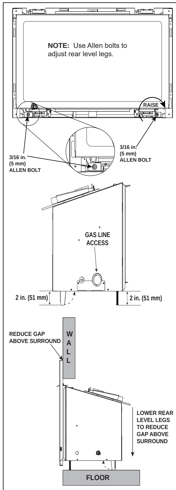
Figure 5.13 Leveling Leg Detail
