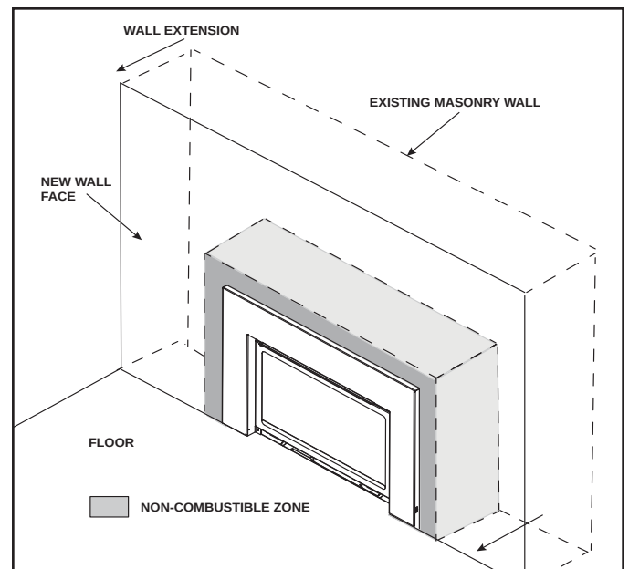
Figure 3.9 Non-Combustible Framing / Facing Requirement
