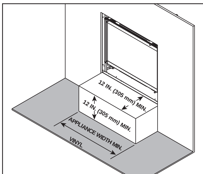
Figure 8.9 Vinyl Flooring Recommendations
