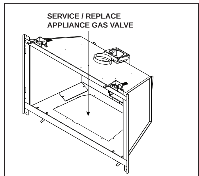
Figure 6.5 Gas Valve Detail
