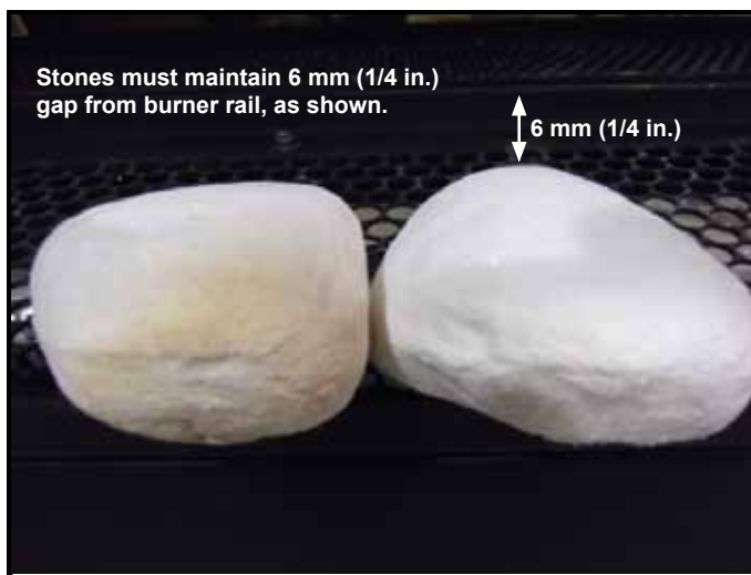
Figure 3. Placement of Media from Burner Rail
