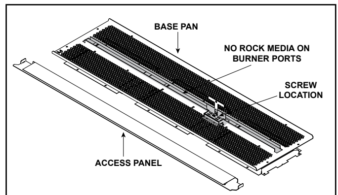
Figure 1. Location of Stone Placement Jig
