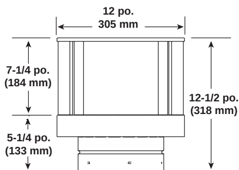
DVP-TVHW Capuchon Vertical (Grand vent)
