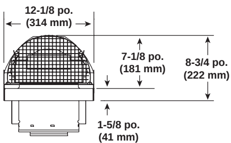
DVP-HPC Capuchon haute performance
