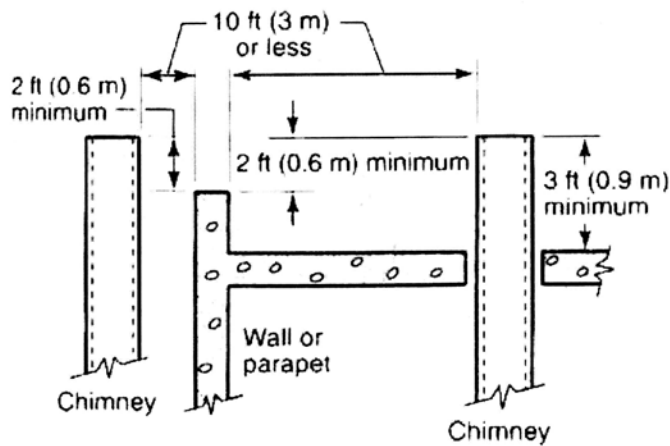
(a) Termination 10 ft (3 m) or less from ridge, wall, or parapet
