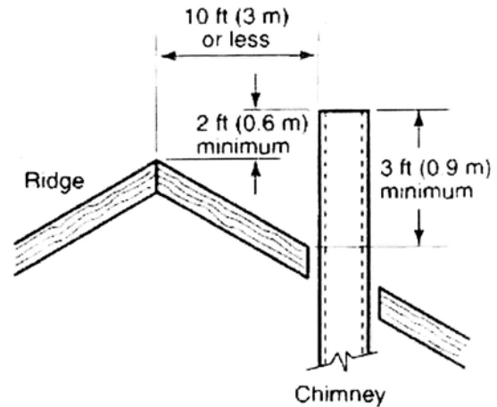
(a) Termination 10 ft (3 m) or less from ridge, wall, or parapet
