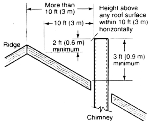
(b) Termination more than 10 ft (3 m) from ridge, wall, or parapet
