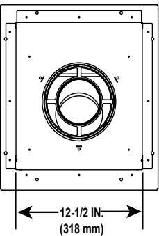
Figure 11.5 Vent Components
