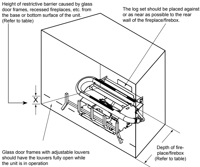
Figure 2.2 - Reference Drawing of a EYF-B Log Set in an Enclosure with Glass Door or Barrier Installed
