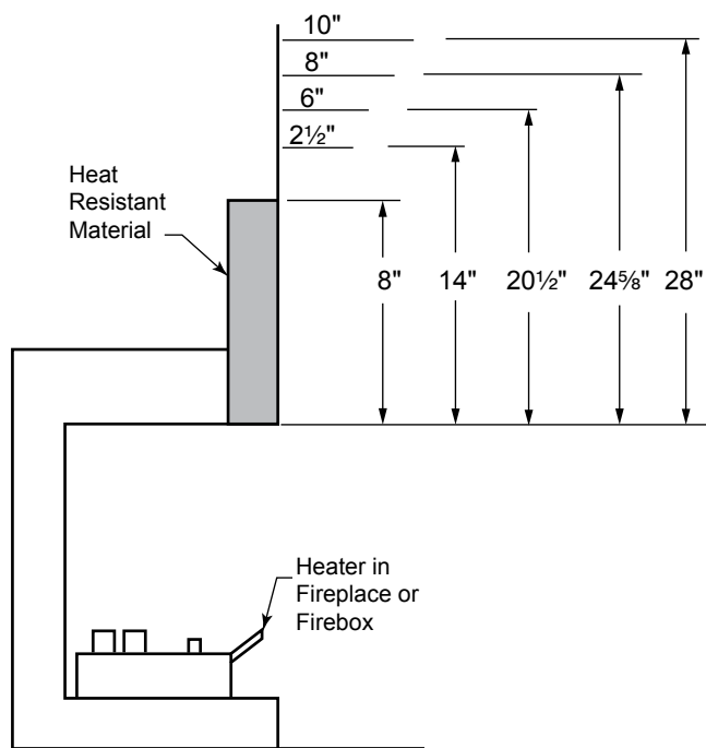
Figure 3.4 - Minimum Mantel Clearance with No Hood
