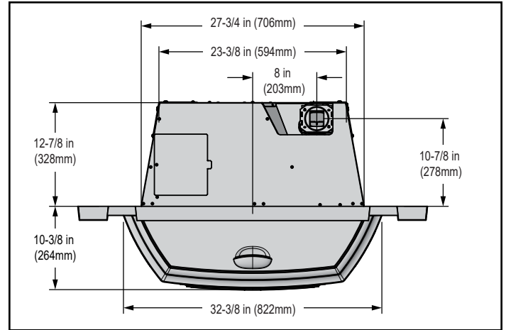
Figure 8.4 - Top View with Cast Panel Set
