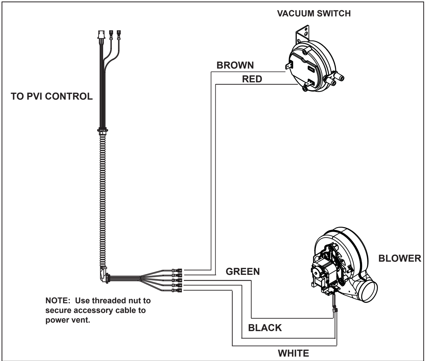
Figure 5. Internal PVI Wiring
