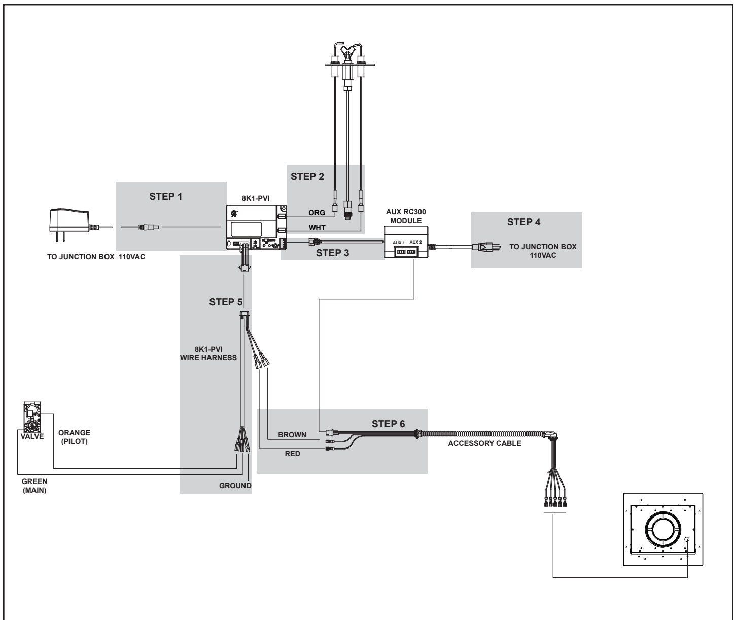
Figure 4 PVI Wiring for RC-MLT, SMART-STAT and SMART-BATT
