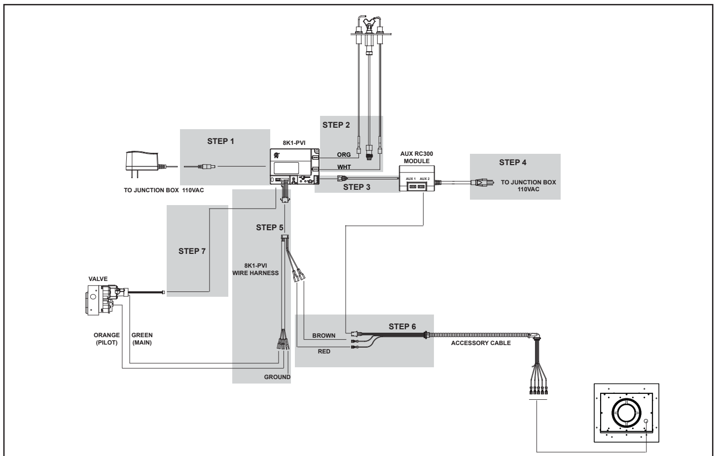
Figure 3 PVI Wiring for RC100, RC200, RC300 Controls
