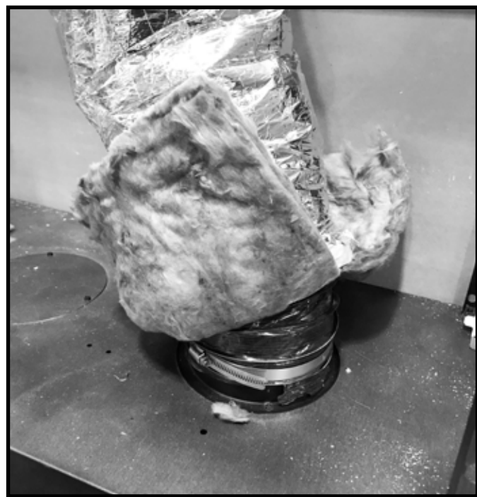
Figure 5.14 Install Flex Venting to Appliance
