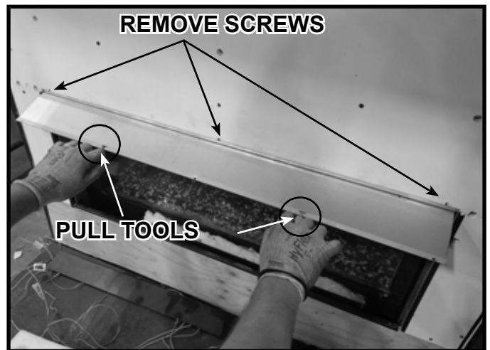
Figure 5.7 Use Pull Tools to Remove Heat Shield
