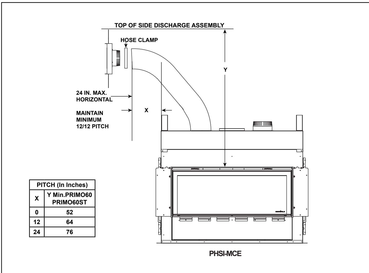
Figure 3.1 Side Discharge - Maintain Pitch
