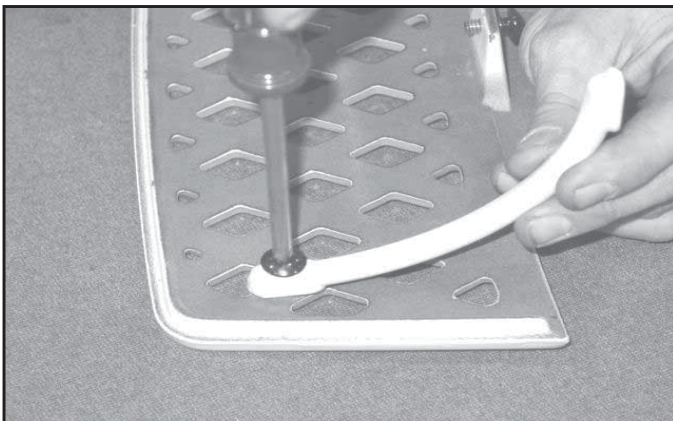
Figure 2. Install Warming Shelf Bracket
