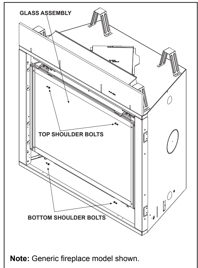
Figure 1. Install Shoulder Bolts
