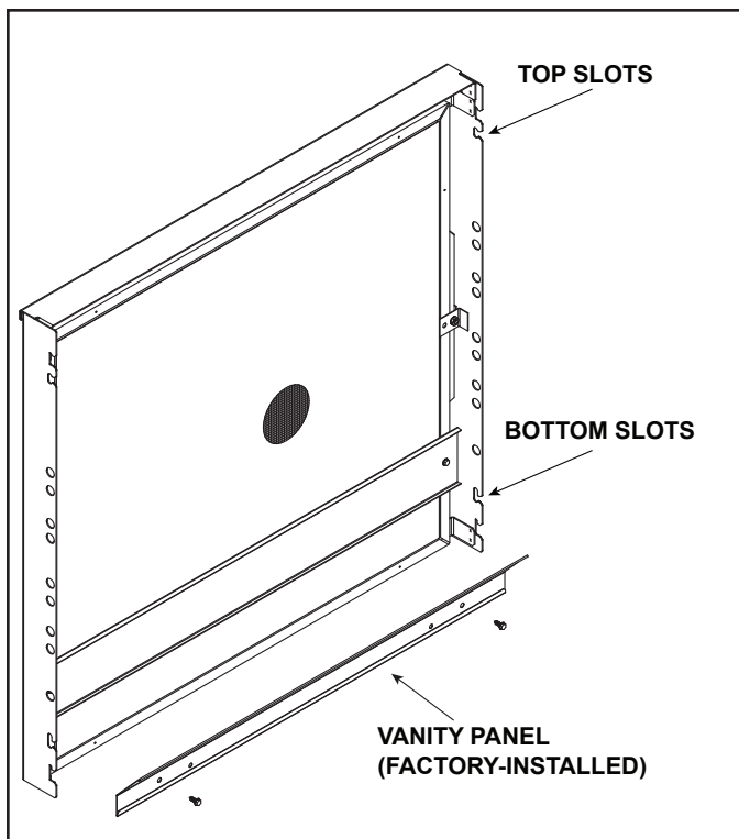
Figure 2. Install Vanity Panel on Folio Decorative Front
