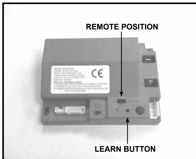
Figure 7. Programming RC300CE
