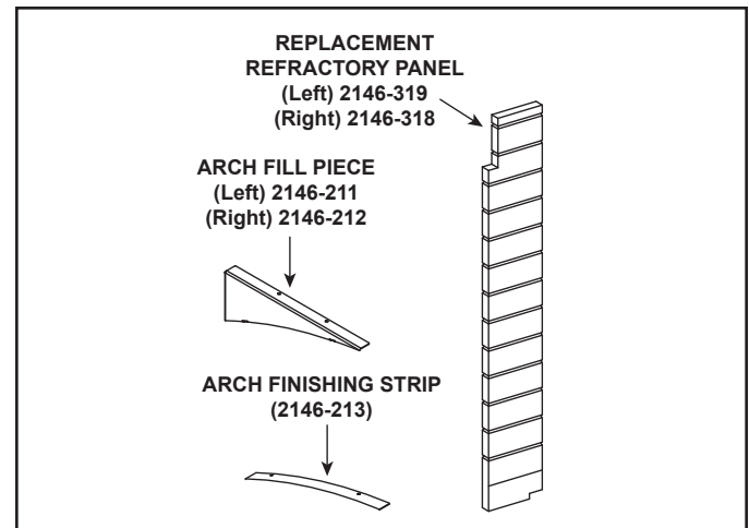
Figure 1. ARCHKIT-ESC42ST Contents
