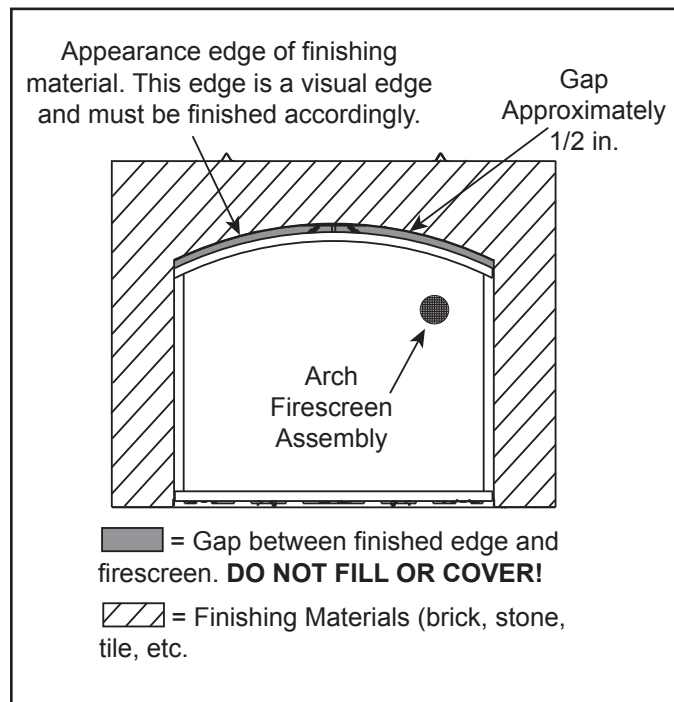
Figure 7. Finishing detail
