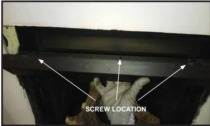
Figure 3. Top Baffle Placement
