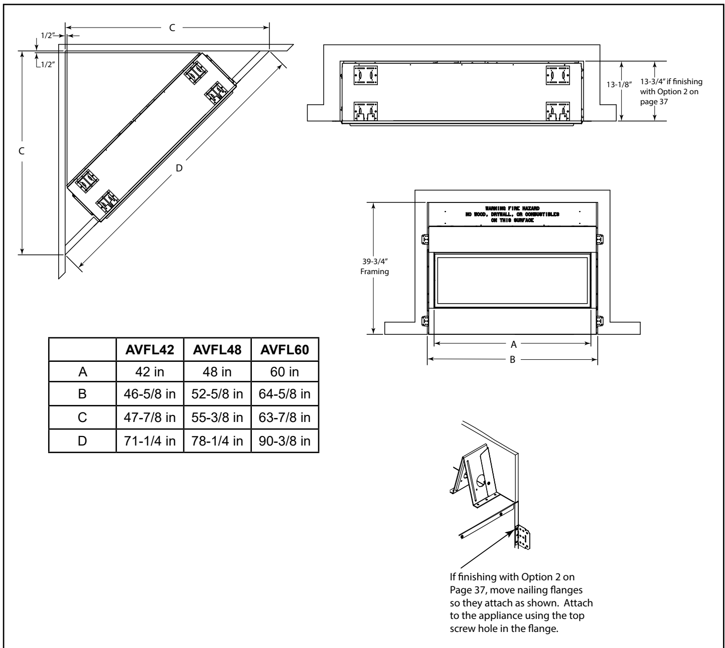
Figure 3.4 - Framing Dimensions
