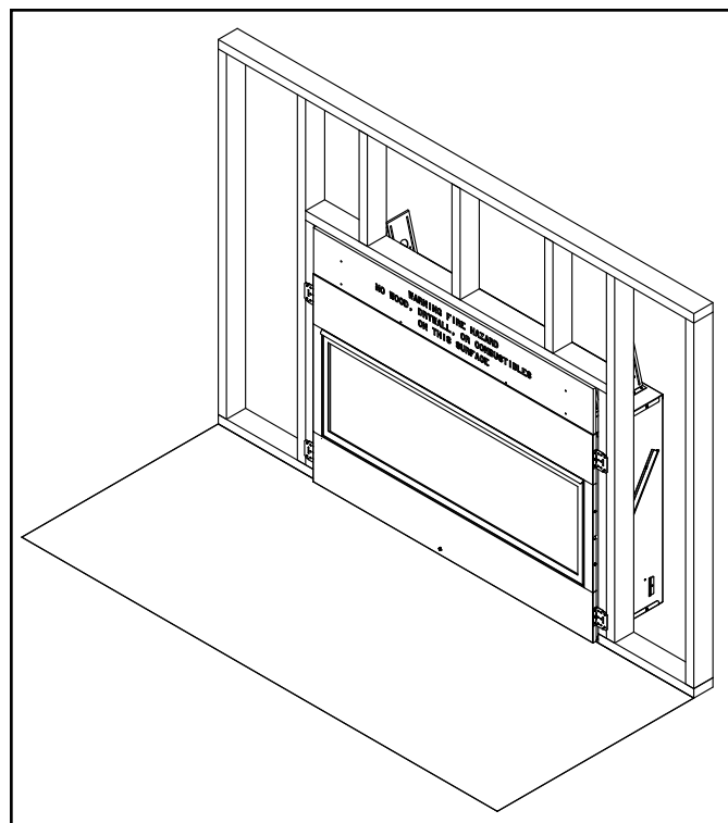
Figure 3.12 - Floor Protection
