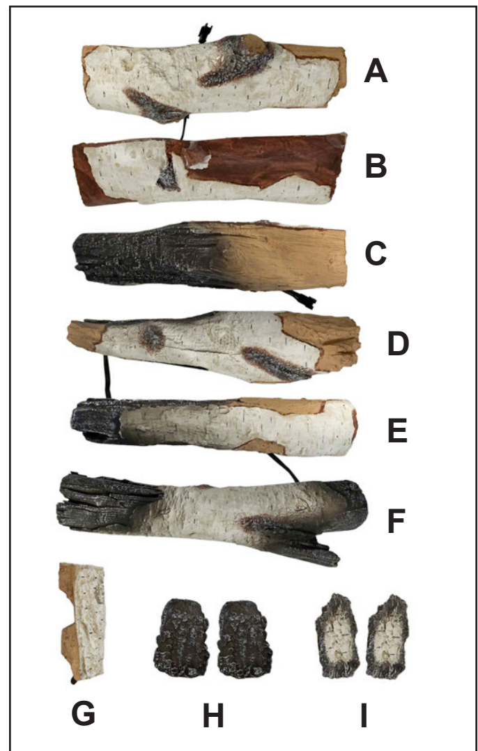
Figure 1. SF-ALLH-BIRCH Logs
