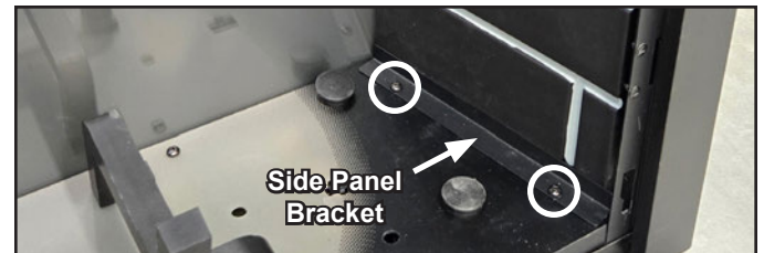
Figure 2 Side Panel Bracket Screws
