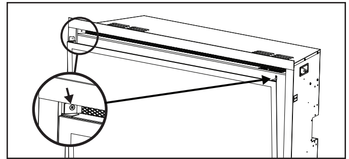
Figure 1 Front Glass Attachment Screws
