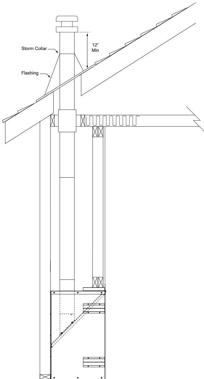
PL Vent Pipe installed through a ceiling.
