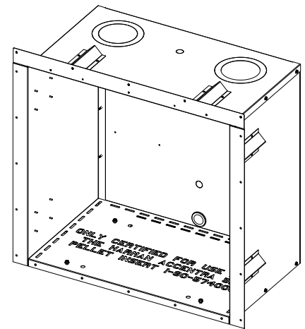
Zero Clearance Cabinet
