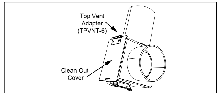
Figure 21.4 - Rear to Top Vent Adapter - 90°
