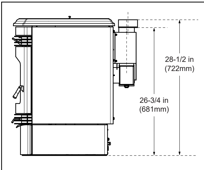
Figure 9.2 - Side View with Top Vent Adapter (TPVNT-2) and Offset Adapter (811-0720).
