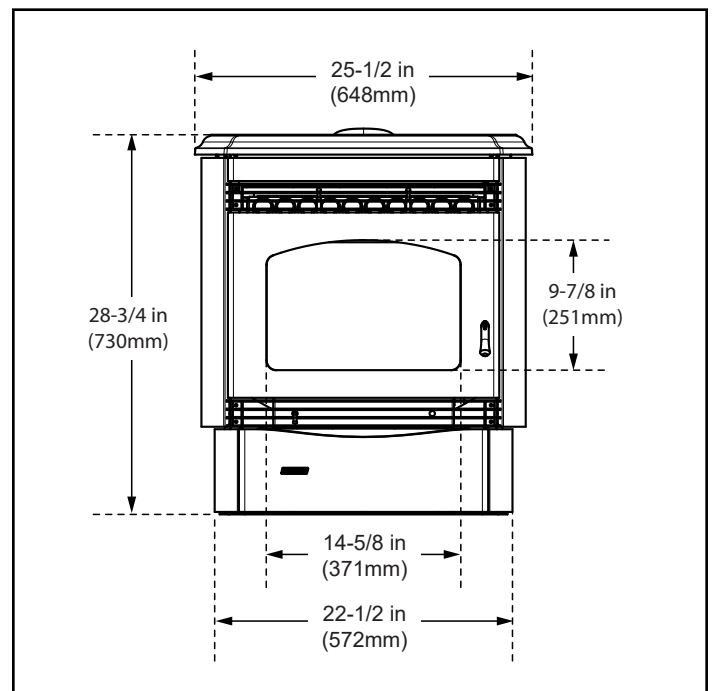
Figure 8.4 - Front View
