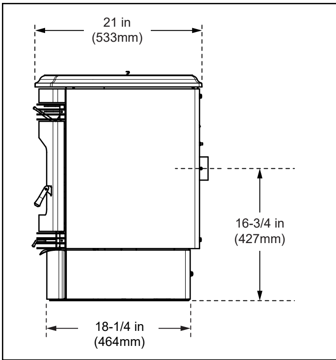
Figure 9.1 -Side View
