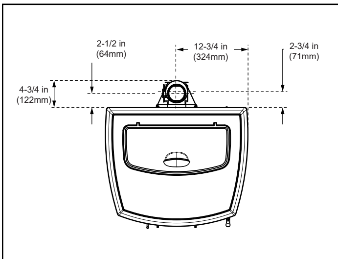
Figure 8.2 - Top View with Top Vent Adapter (TPVNT-2) and Offset Adapter (811-0720).
