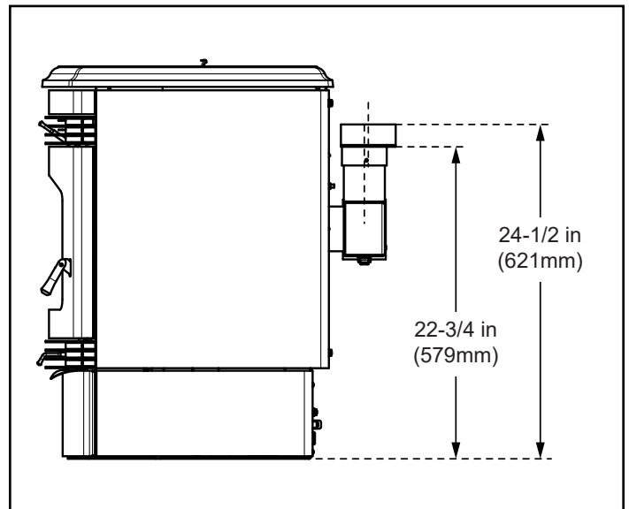
Figure 9.4 - Side View with Top Vent Adapter (TPVNT-6) and Offset Adapter (811-0720).
