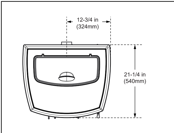
Figure 8.1 - Top View
