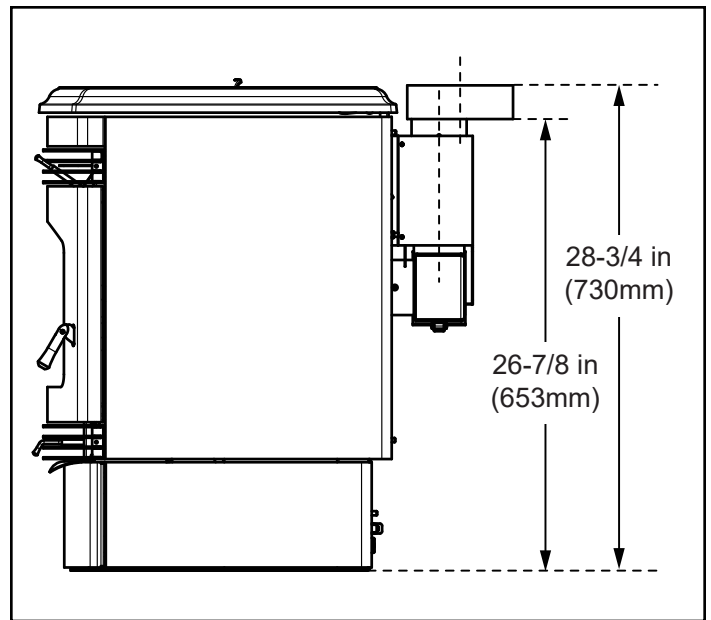
Figure 9.3 - Side View with Top Vent Adapter (TPVNT-2) and Offset Adapter (812-3570).
