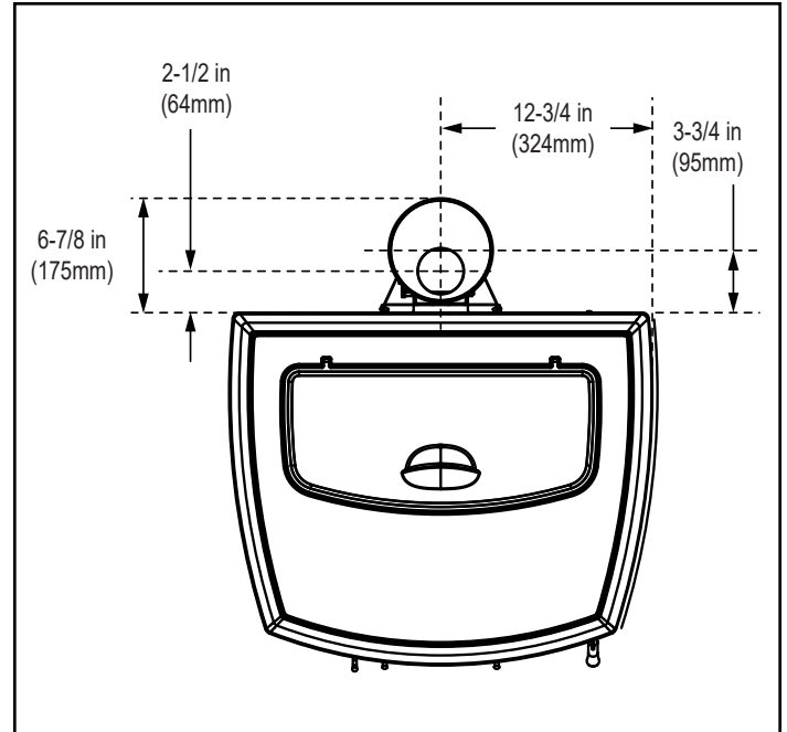
Figure 8.3 - Top View with Top Vent Adapter (TPVNT-2) and Offset Adapter (812-3570).
