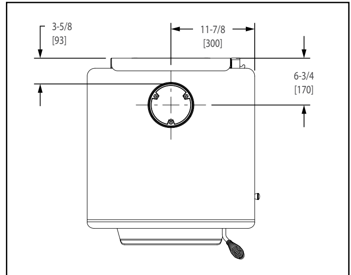
Figure 8.2 - Top View
