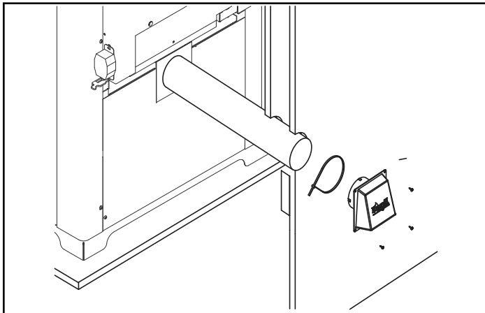
Figure 16.1 - Rear Installation
