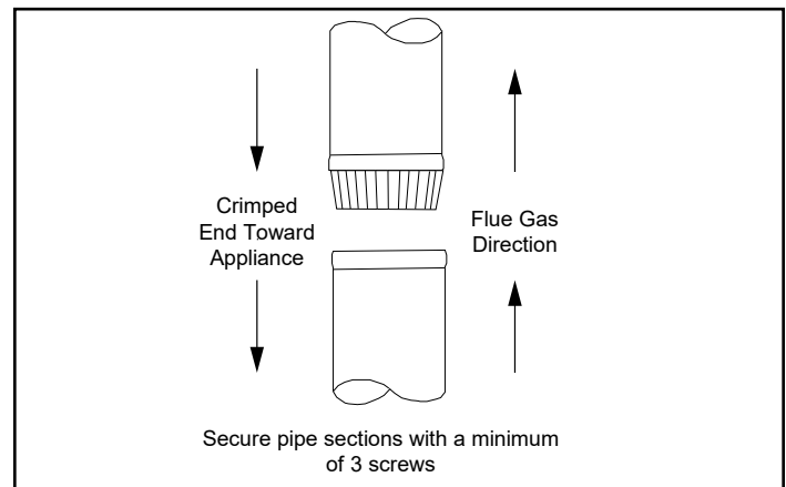
Figure 20.3 - Chimney Connector (Appliance Pipe)
