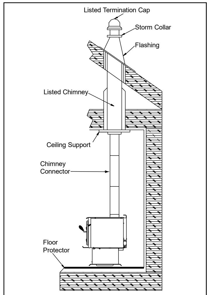
Figure 19.1 - Prefabricated Interior Chimney
