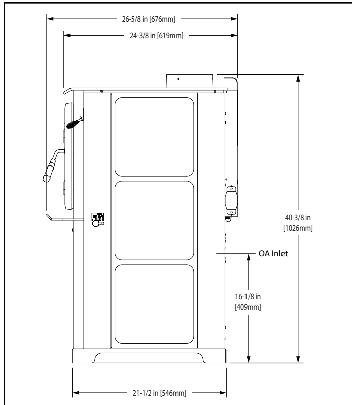
Figure 8.3 - Side View
