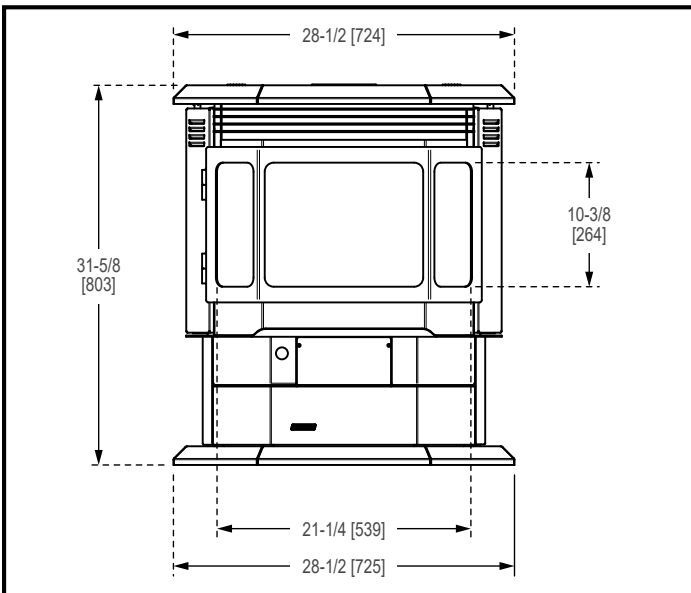
Figure 8.3 - Front View
