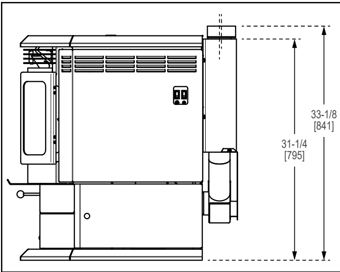
Figure 9.1 - Side View with Top Vent Adapter (TPVNT-1) and Offset Adapter (811-0720)
