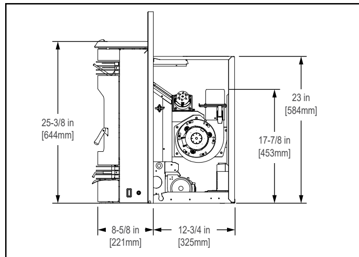
Figure 8.3 - Side View
