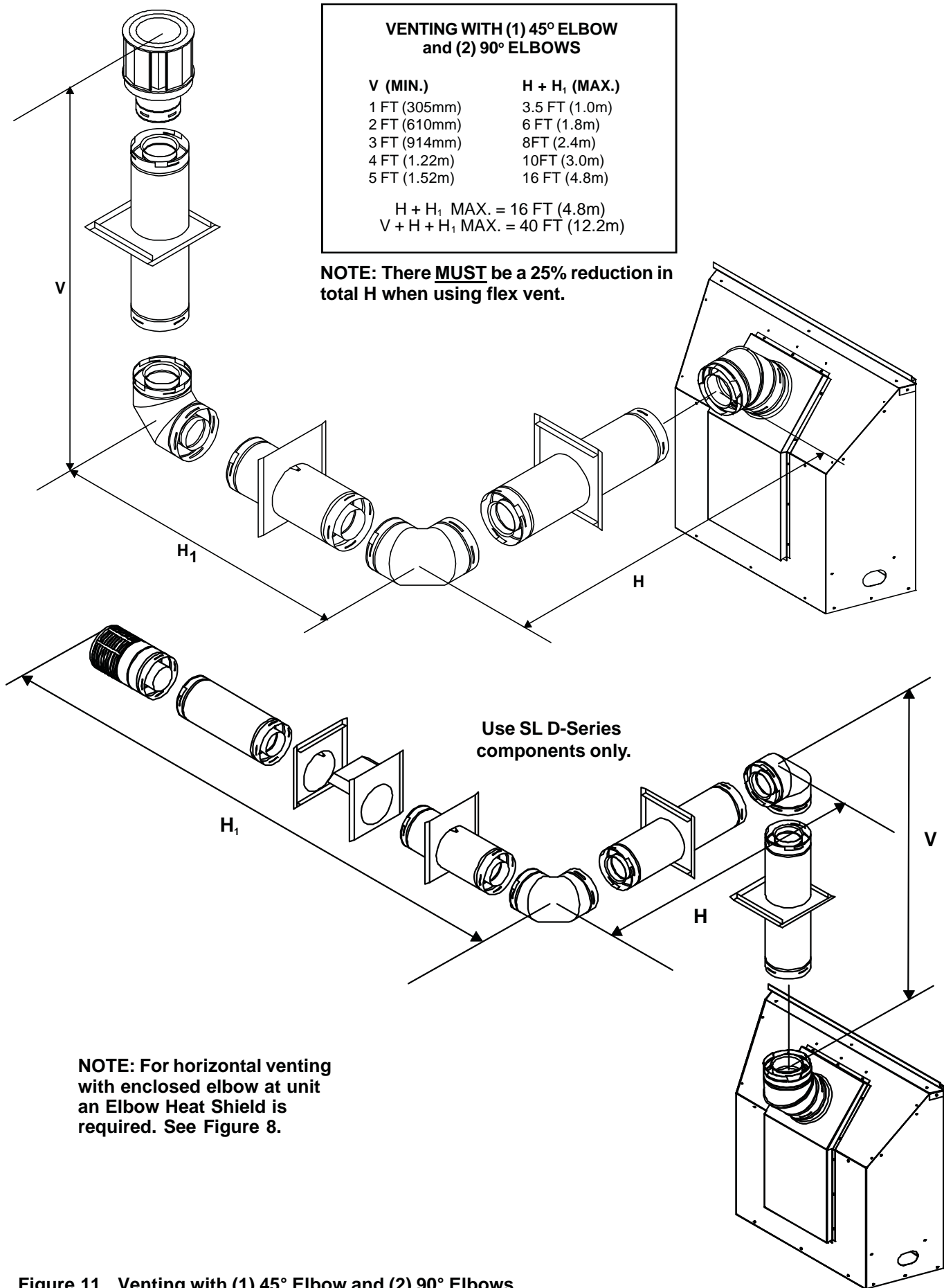
Figure 11. Venting with (1) 45° Elbow and (2) 90° Elbows.
