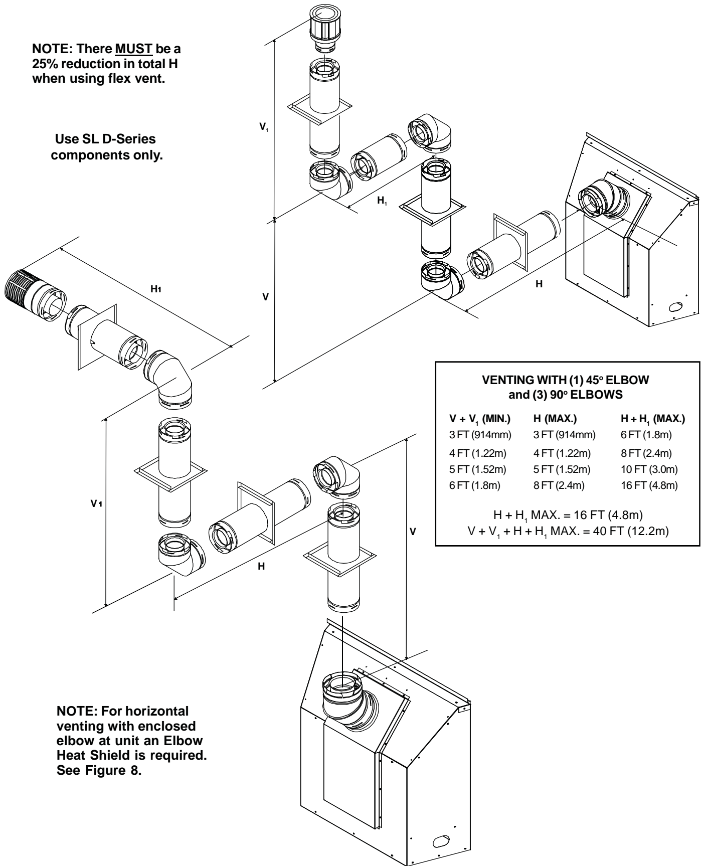
Figure 10. Venting with (1) 45° Elbow and (3) 90° Elbows.
