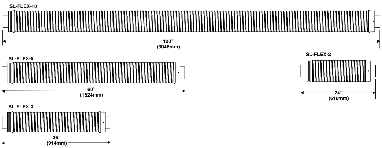
Figure 4. NOTE: PIPES OVERLAP 1-3/8 INCHES (34.93mm) AT EACH JOINT. SL-Series and SL-Flex Series Direct Vent Component Specifications (4-inch inner pipe / 6 5/8-inch outer pipe)
