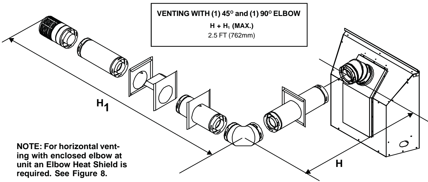
Figure 9. Venting with (1) 45° Elbow and (1) 90° Elbow.
