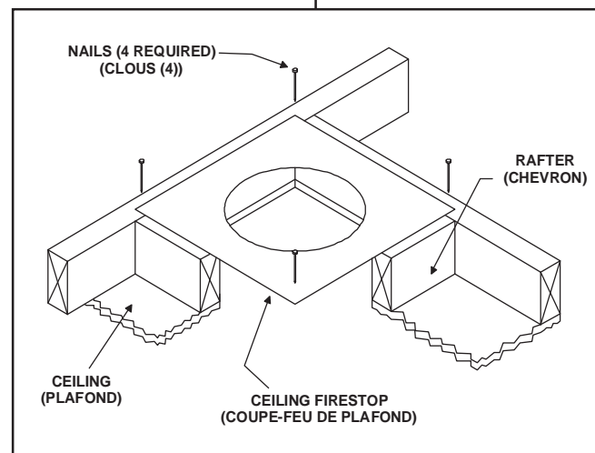
Figure 18. Attic Firestop
