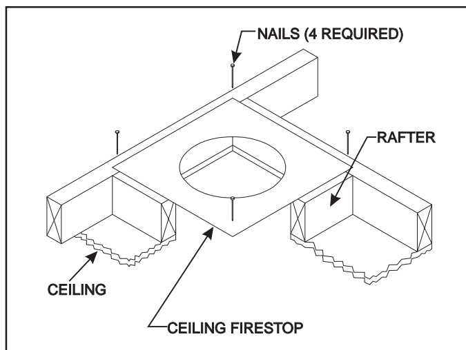
Figure 18. Attic Firestop
