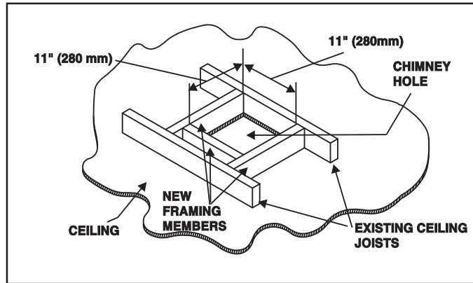
Figure 16. Hole and New Framing Members
