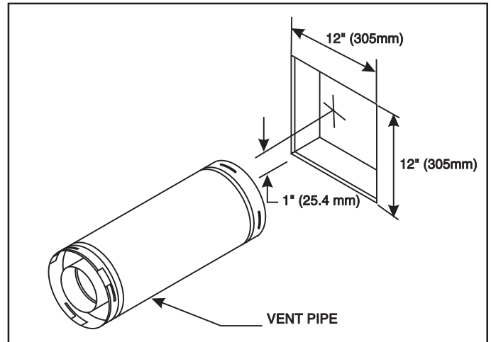
Figure 14. Hole and Vent Pipe
