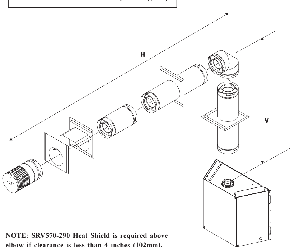
Figure 7. Venting with One 90° Elbow
