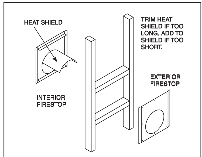
Figure 15. Heat Shield, Interior and Exterior Firestops
