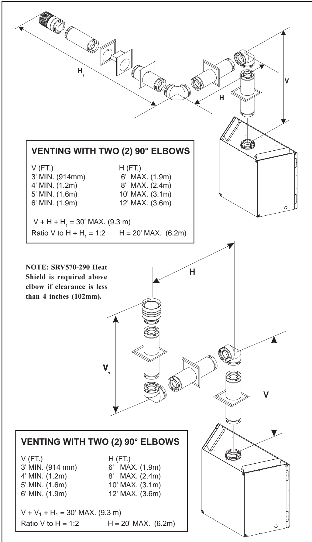
Figure 8. Venting with two 90° elbows
