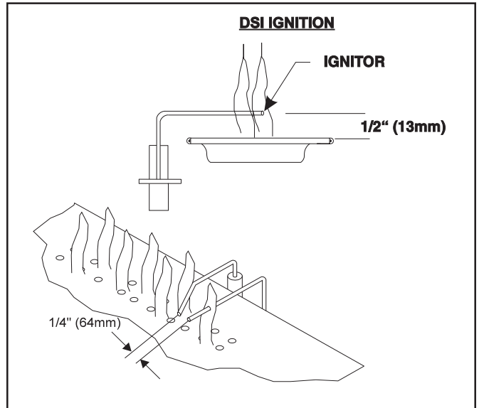
Figure 24. Gas Controls Systems
