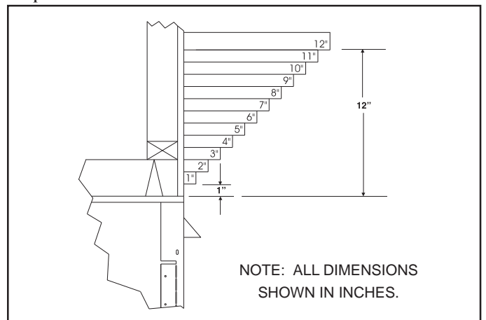
Figure 28. Minimum Vertical and Maximum Horizontal Dimensions of Combustibles above Fireplace
