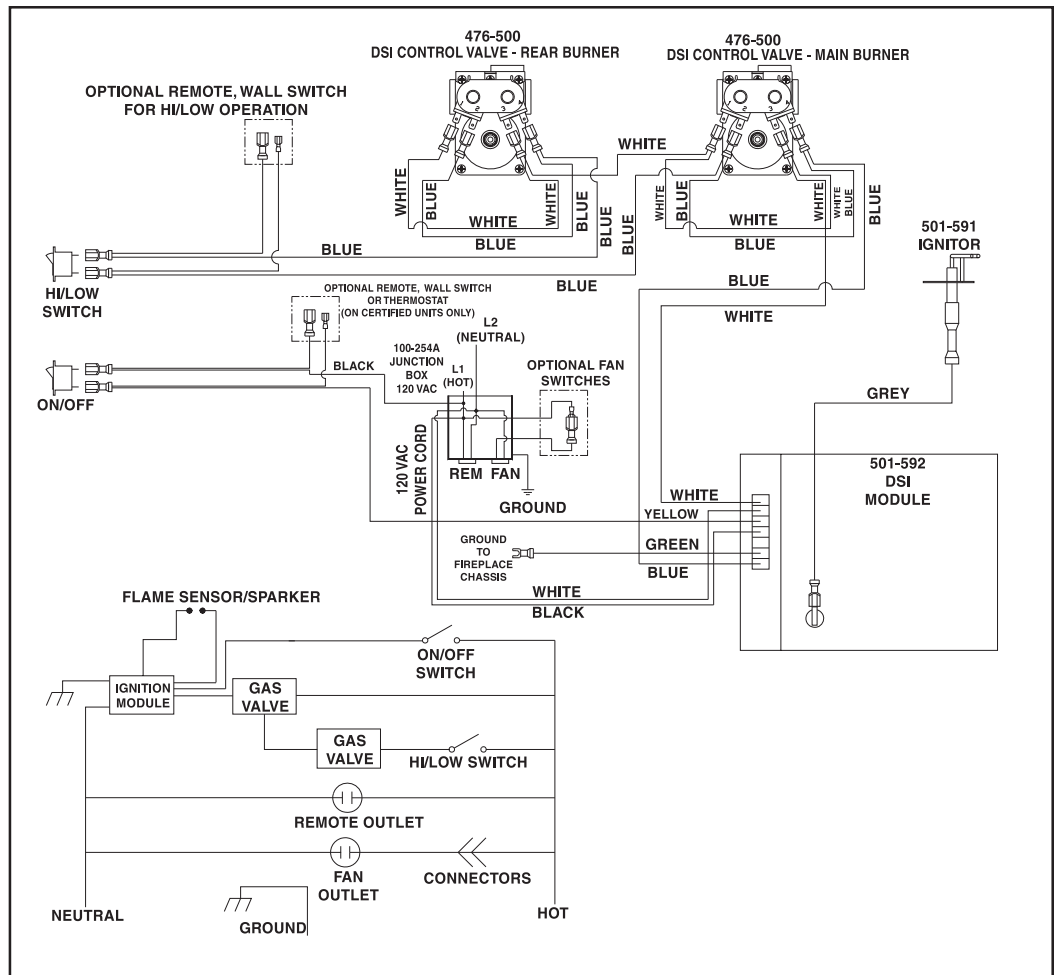
Figure 27. Direct Spark Ignition (DSI) Wiring Diagram
