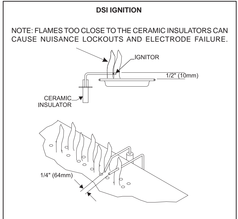
Figure 33. Ignitor Flame Patterns
