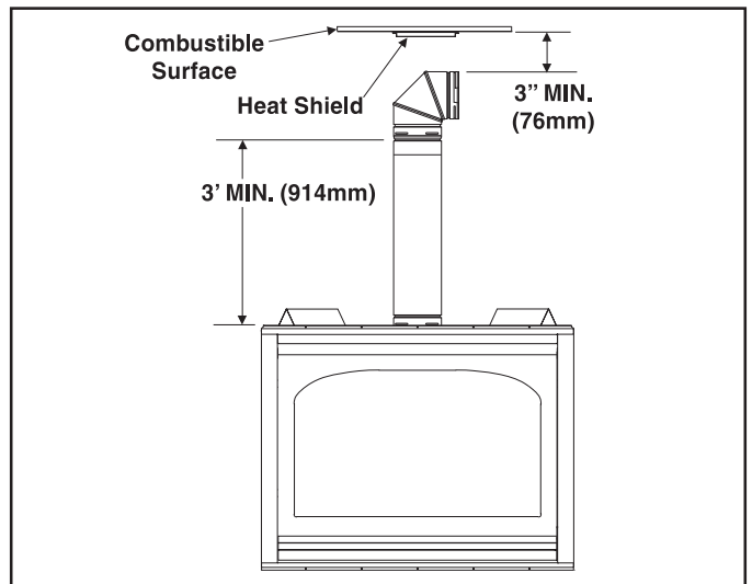
Figure 12. Placement of SRV570-290 Heat Shield First 90 elbow in system.
