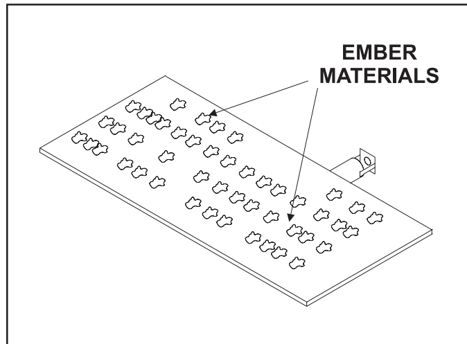
Figure 31. Follow placement of the ember material
