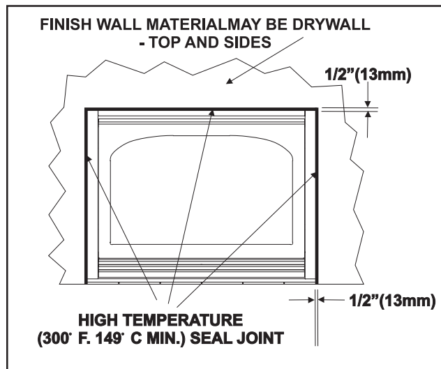
Figure 29. Sealant Material
