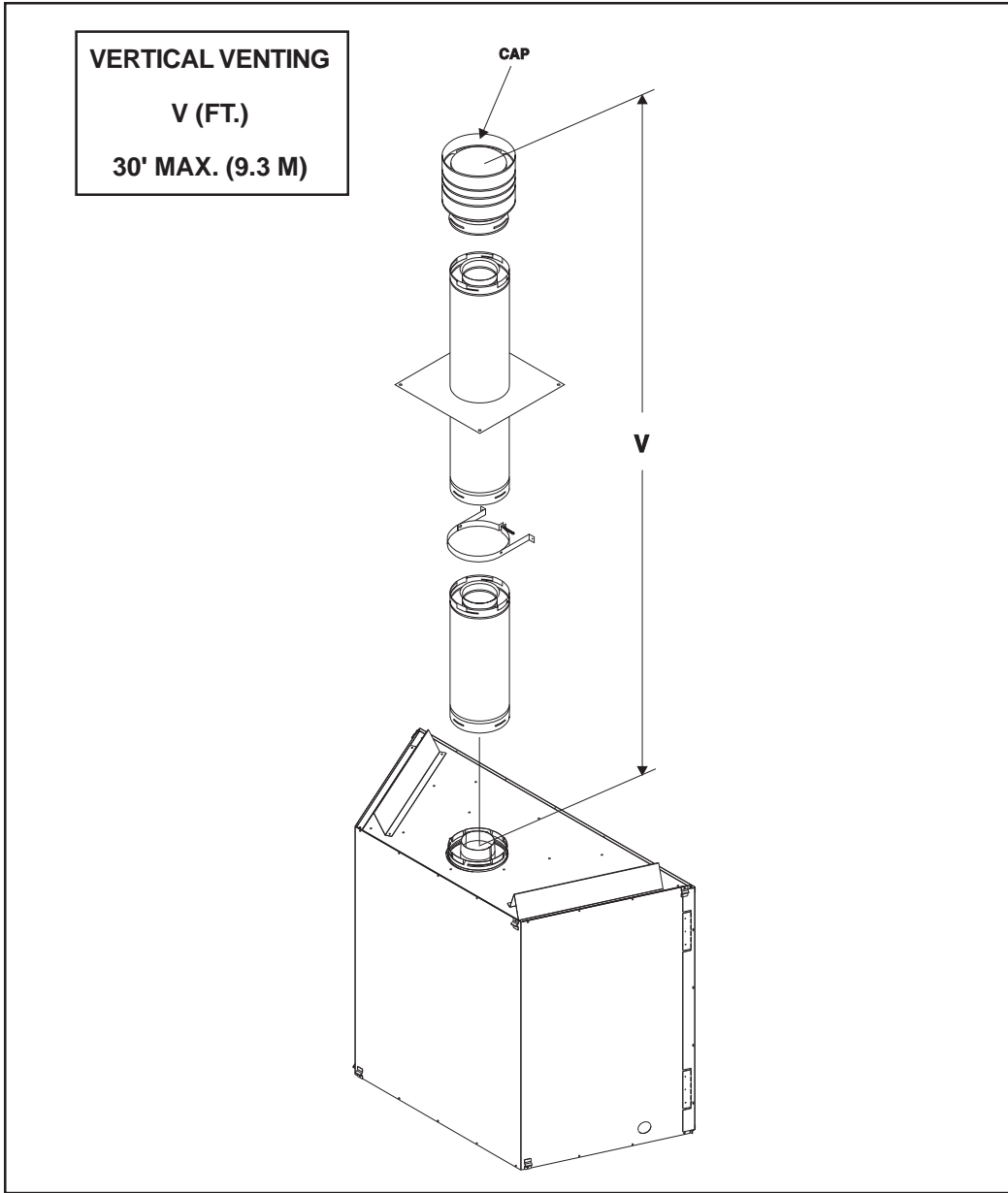
Figure 6. Vertical Venting
