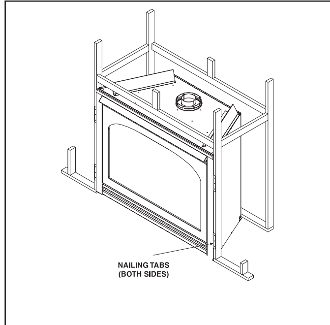
Figure 23. Proper Positioning, Leveling, and Securing of a Fireplace
