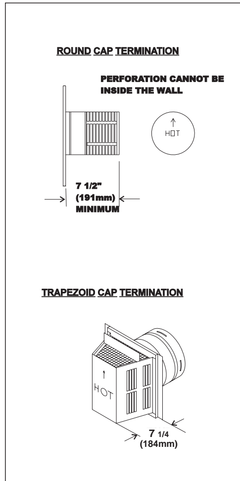
Figure 19. Round and Trapezoid Termination Caps
