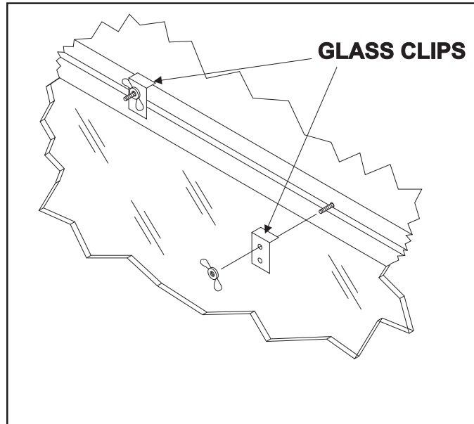
Figure30. Glass Assembly
