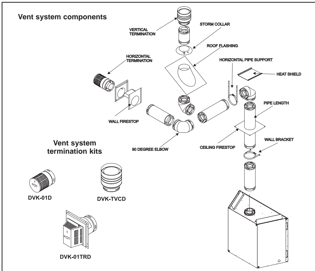
Figure 4. Vent Components and Terminations
