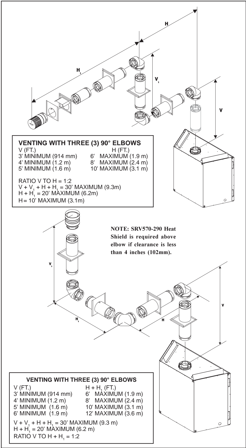
Figure 9. Venting with three 90° elbows
