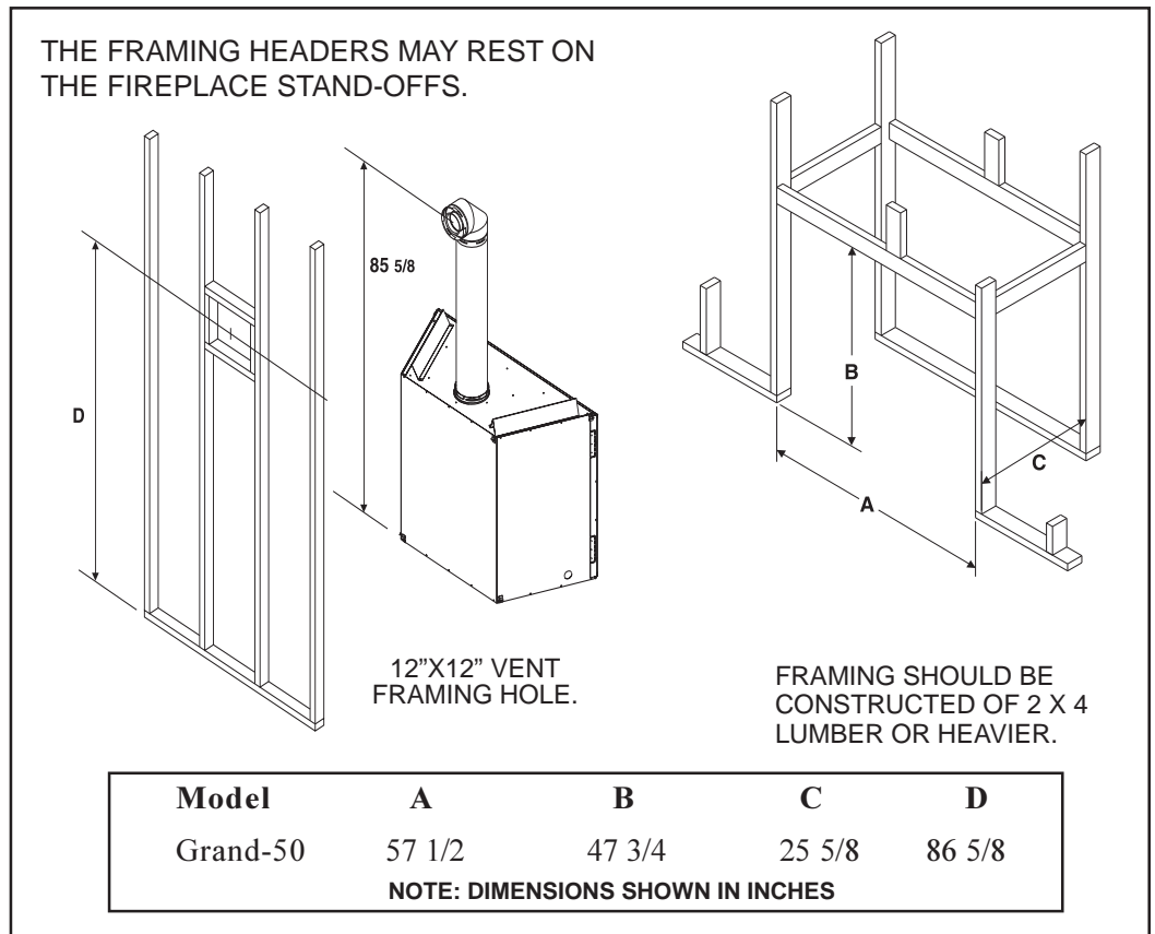
Figure 3. Framing Dimensions
