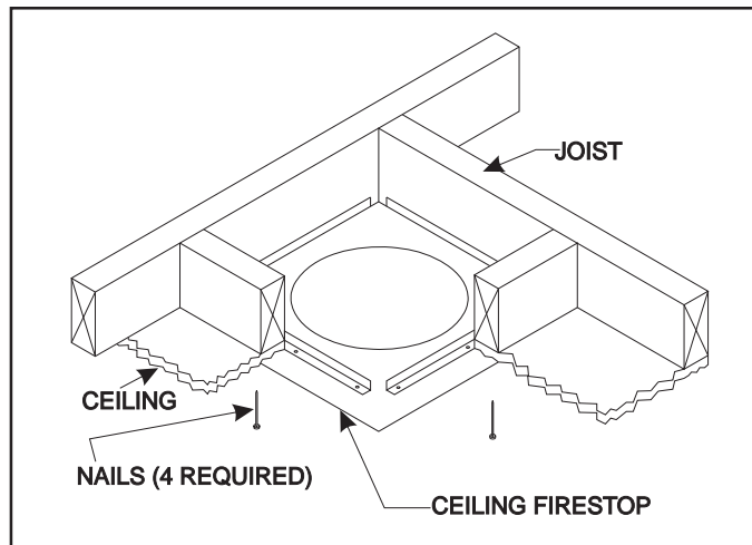
Figure 17. Ceiling Firestop (Ceiling Side)
