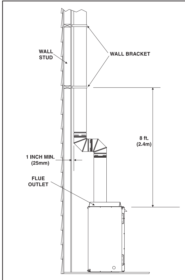
Figure 13. Installing Support Brackets
