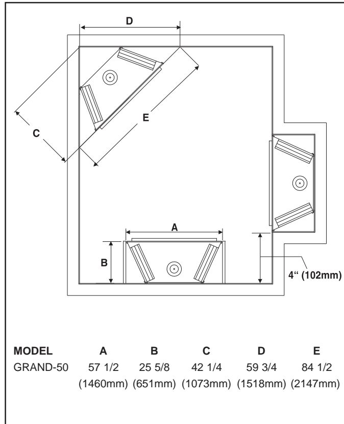
Figure 2. Fireplace Dimensions, Locations, and Space Requirements
