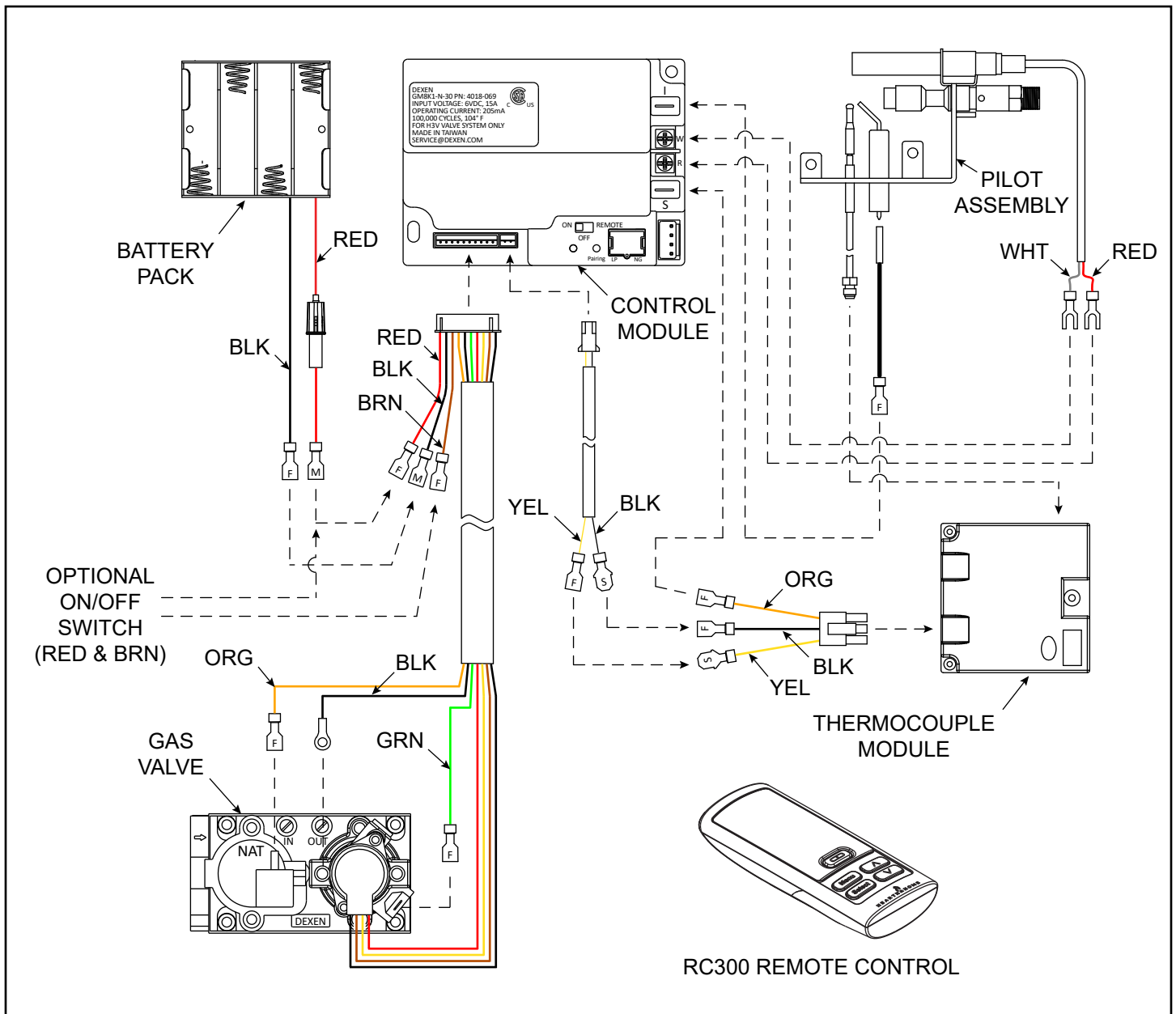
Figure 8.3 Intellifire™ Plus (IPI) Wiring
