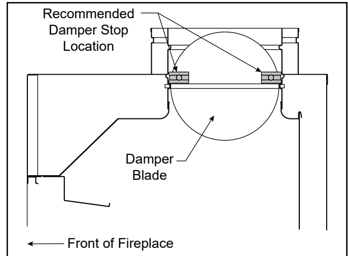
Figure 6.1 Factory-Built Fireplace
