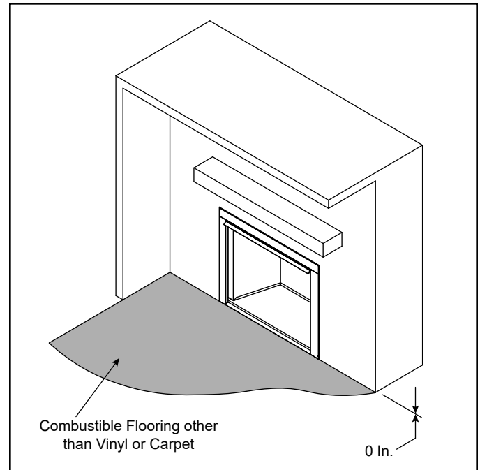
Figure 5.4 Combustible Flooring
