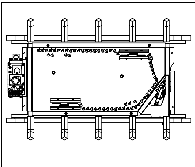
Figure 9.2 Mineral Wool Placement
