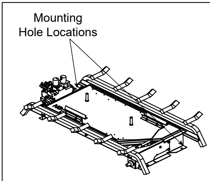
Figure 9.1 Mounting Holes
