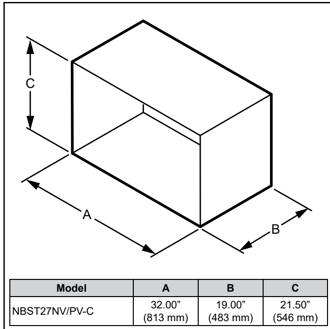
Figure 3.1 Minimum Hearth Dimensions
