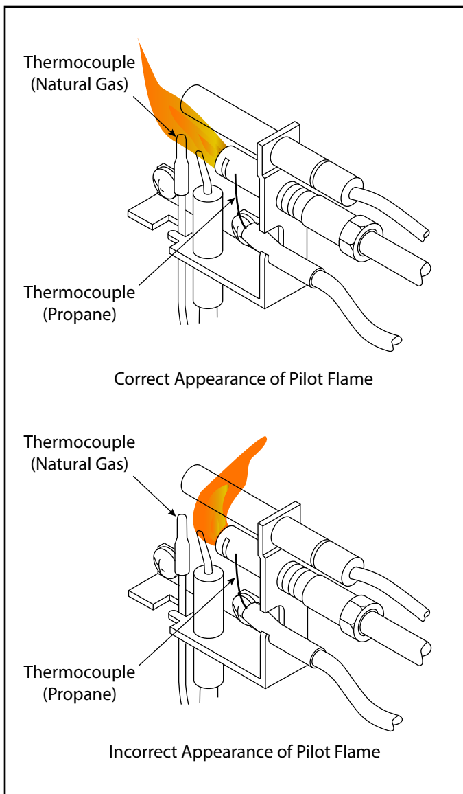
Figure 9.3 Pilot Flame
