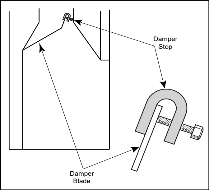
Figure 6.3 Masonry-Built Fireplace
