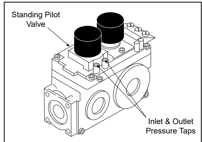
Figure 7.4 Pressure Taps
