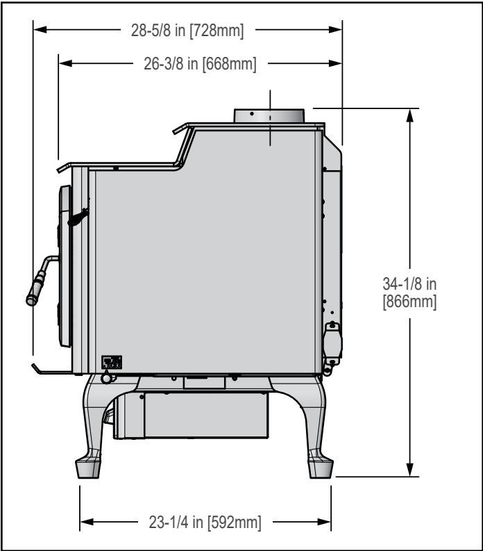
Figure 11.2 - Side View
