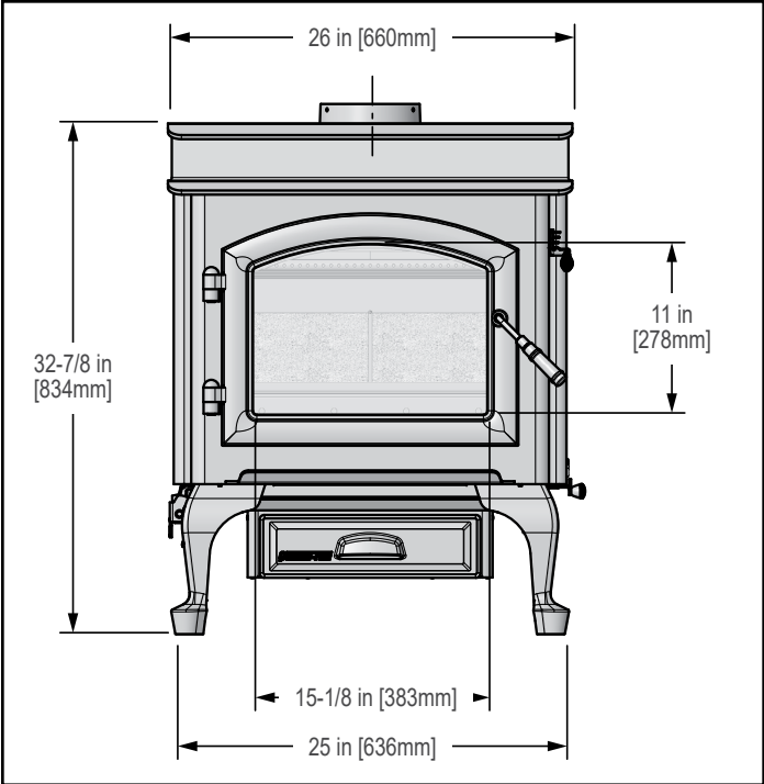
Figure 11.1 - Front View
