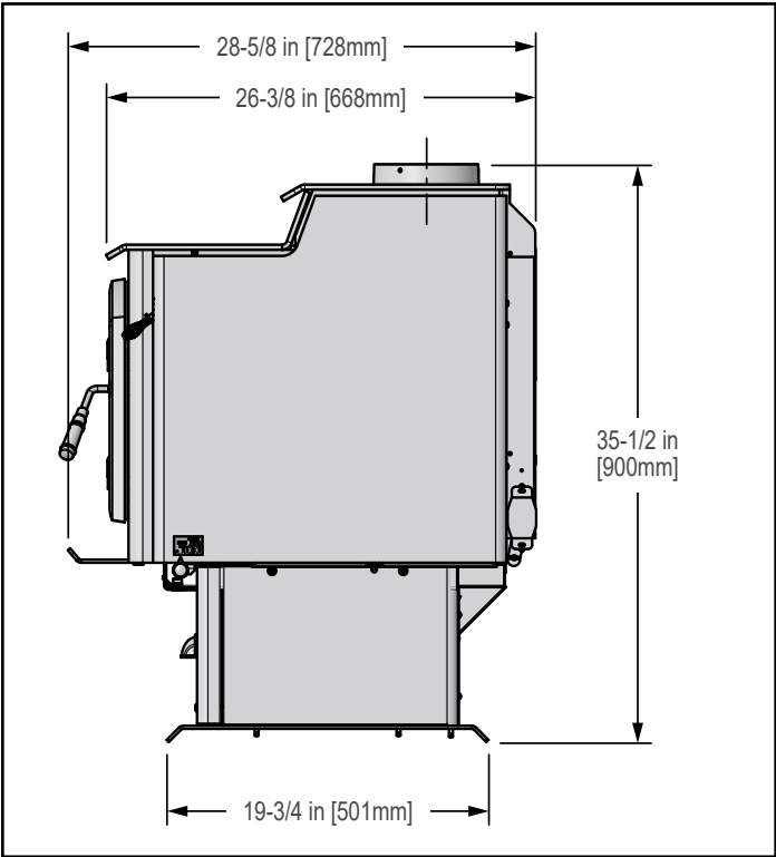
Figure 10.2 - Side View
