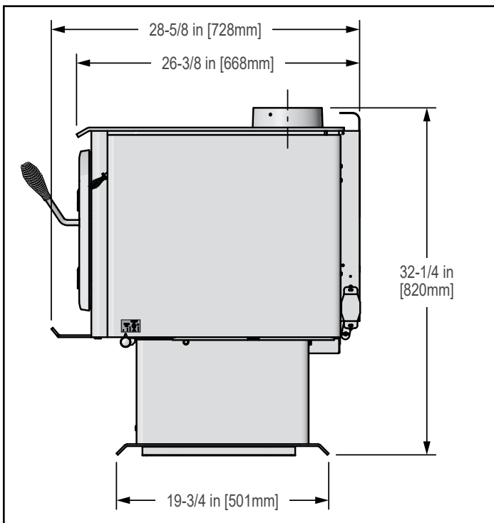
Figure 9.2 - Side View
