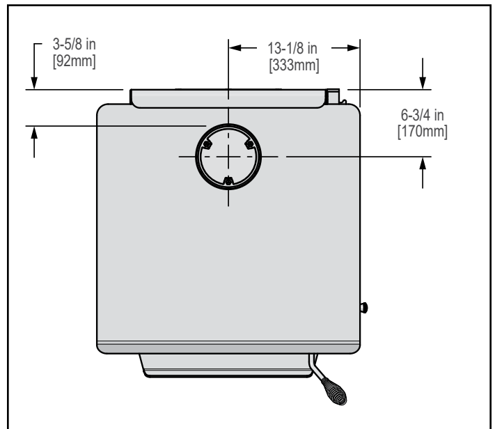
Figure 9.3 - Top View
