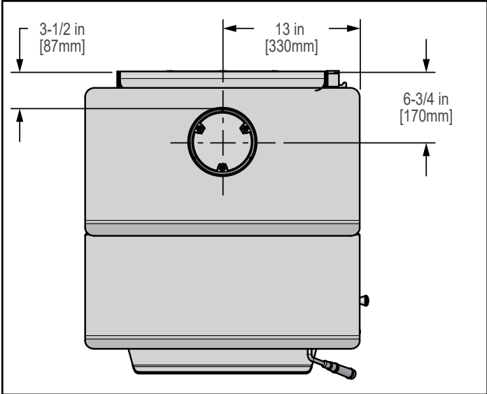
Figure 11.3 - Top View
