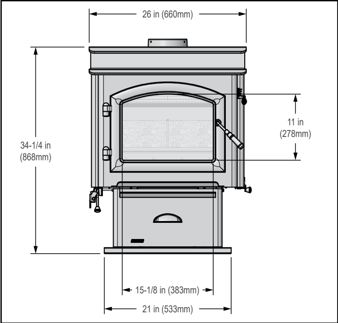
Figure 10.1 - Front View
