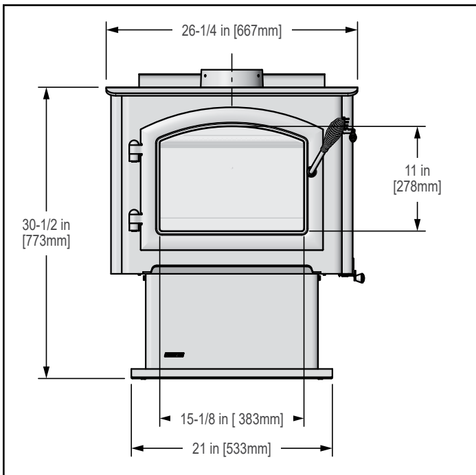
Figure 9.1 - Front View
