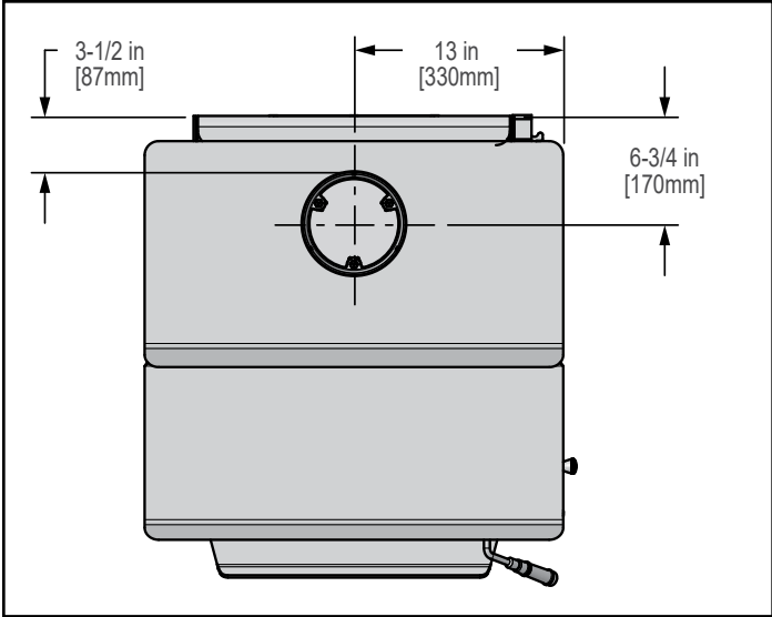
Figure 10.3 - Top View
