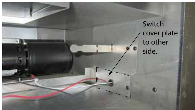
Figure 4.2 Bottom Access Area
