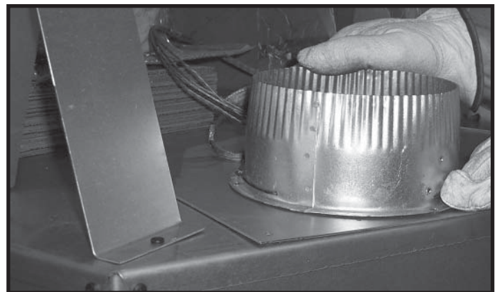
Figure 3. Installing the Round Air Duct
