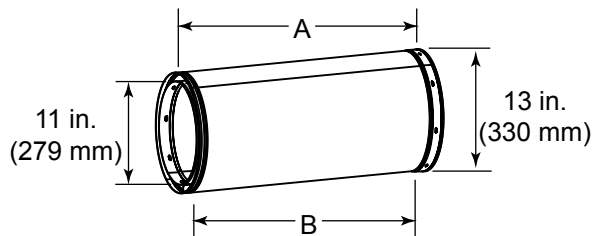
Chimney Sections
