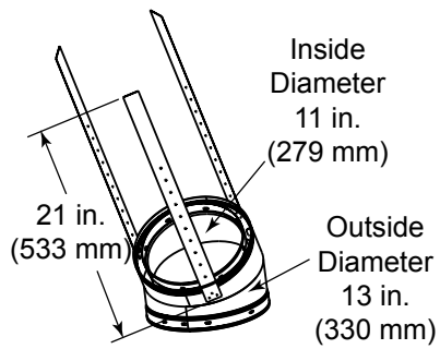
SL1130 Offset/Return
