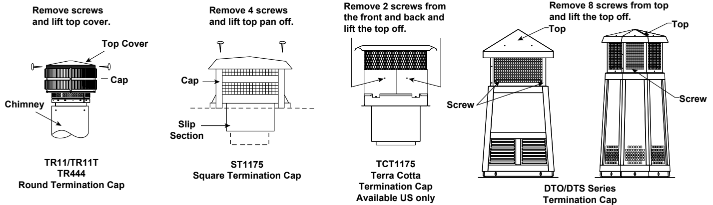
Figure 4.1 Chimney & Termination Cap Cleaning
