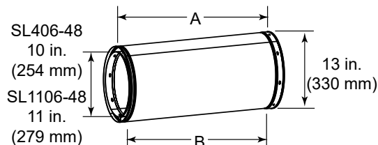
Chimney Sections
