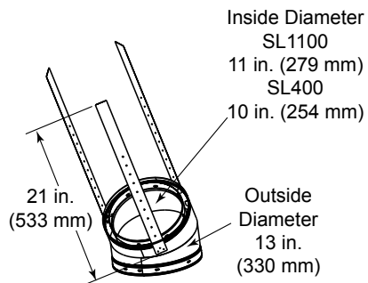
SL1130/SL430 Offset/Return
