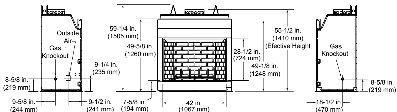
Figure 3.1 Appliance Dimensions
