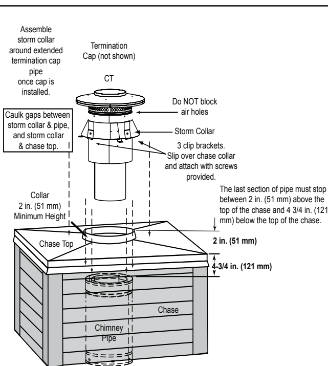
Figure 5.15 Installing a DTO134/DTO146/DTS134/DTS146 Cap
