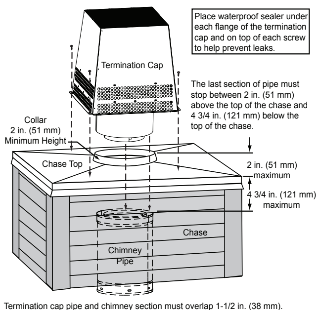
Figure 5.13 Installing a TS345/TS345P Square Termination Cap
