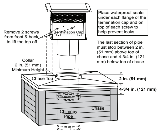
Figure 5.14 Installing a TCT375 Terra Cotta Cap
