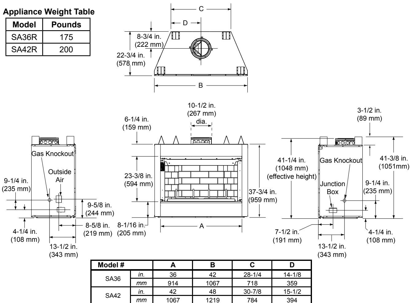
Figure 3.1 Appliance Dimensions
