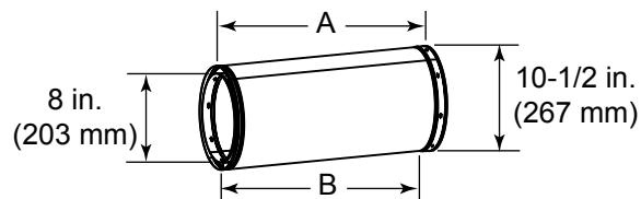
Chimney Sections
