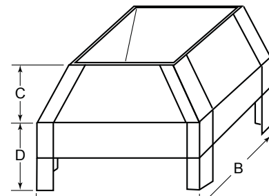
LDS33/LDS46 Decorative Shroud
