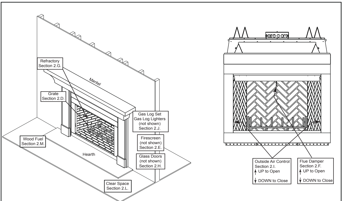
Figure 2.1 General Operating Parts
