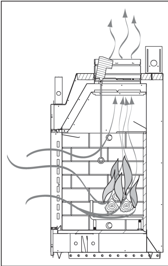
Figure 26 - Flue Draft
