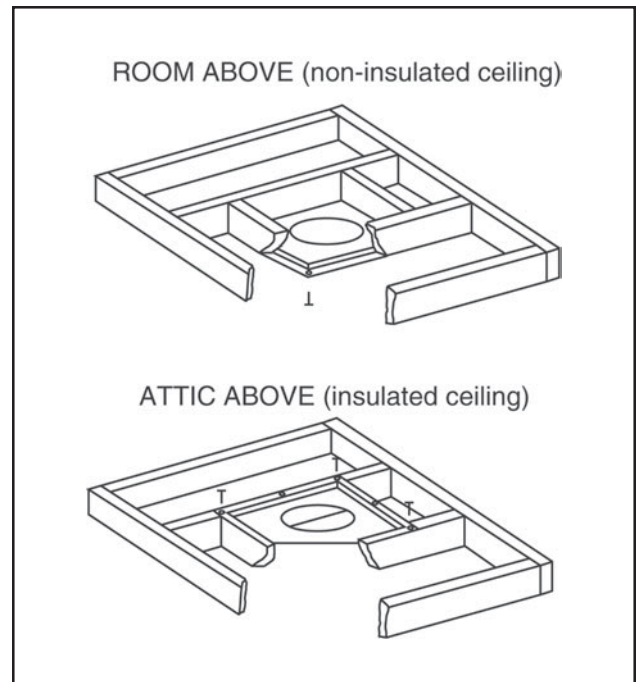
Figure 11 Installing the Firestop Spacer
