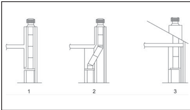
Figure 20 - Chase Constructions
