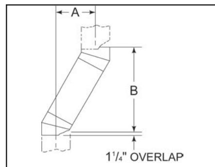
Figure 7 - Chimney Offset/Return
