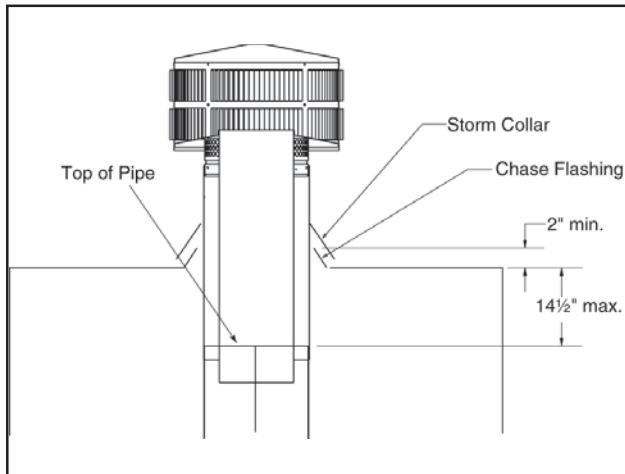
Figure 23 - Installing a TR11T Round Telescoping Termination Cap
