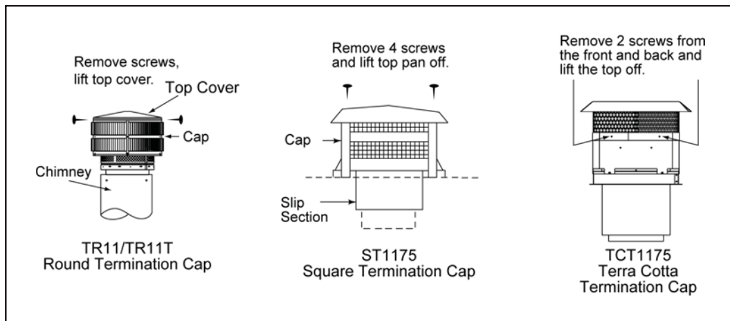
Figure 27 ➔ Chimney & Termination Cap Cleaning
