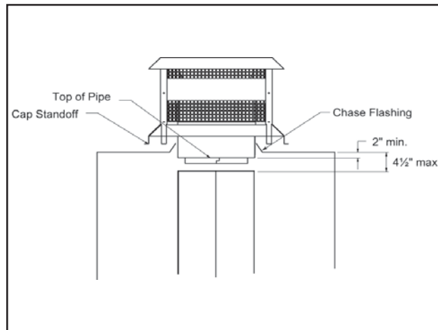
Figure 24 - Installing an ST1175 Square Termination Cap
