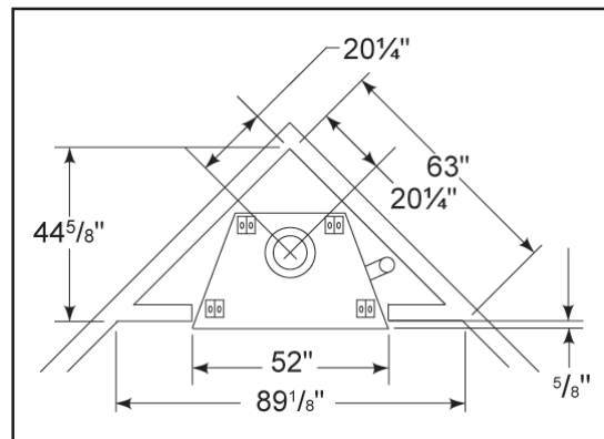
Figure 4 Corner Installation
