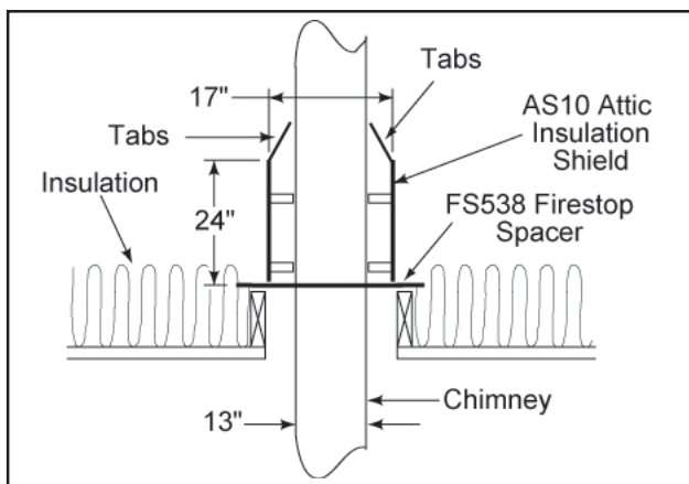
Figure 12 - Installing an Insulation Shield
