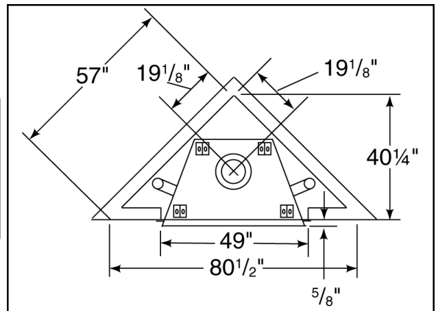
Figure 4 - Corner Installation
