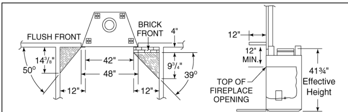
Figure 6 - Sidewalls and Surrounds
