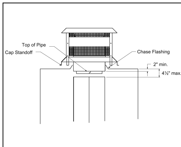
Figure 16 Installing an ST1175 Square Termination Cap
