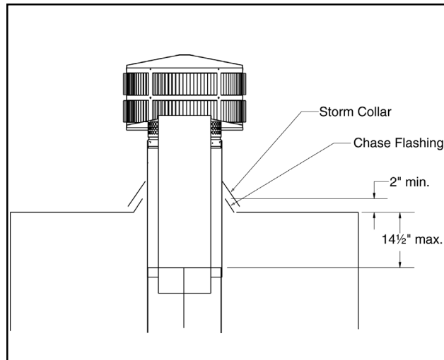
Figure 15 - Installing a TR11T Round Telescoping Termination Cap
