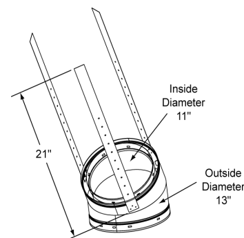
SL1130 - Offset/Return
