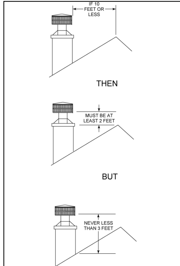
Figure 8 - Chimney Height
