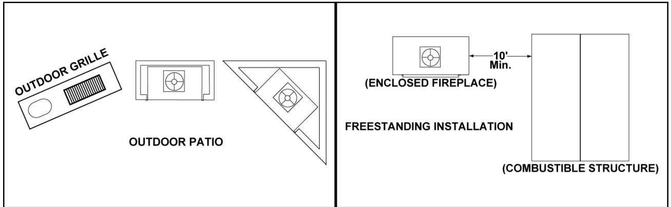
Figure 2 - Fireplace Locations
