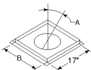
Firestop Spacer
