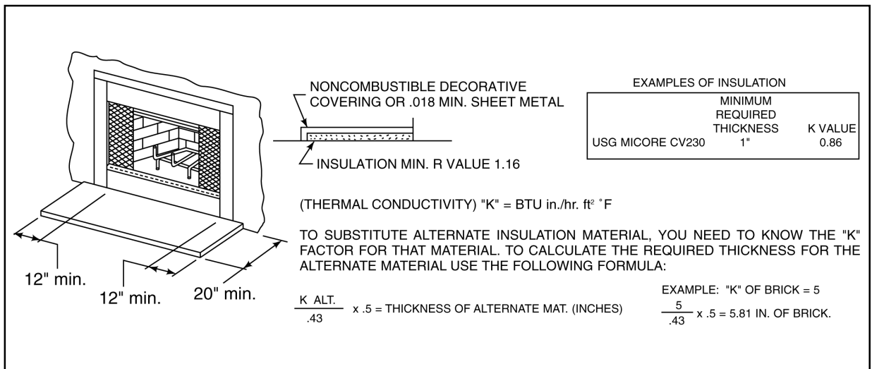
Figure 22 - Field Constructed Hearth Extension
