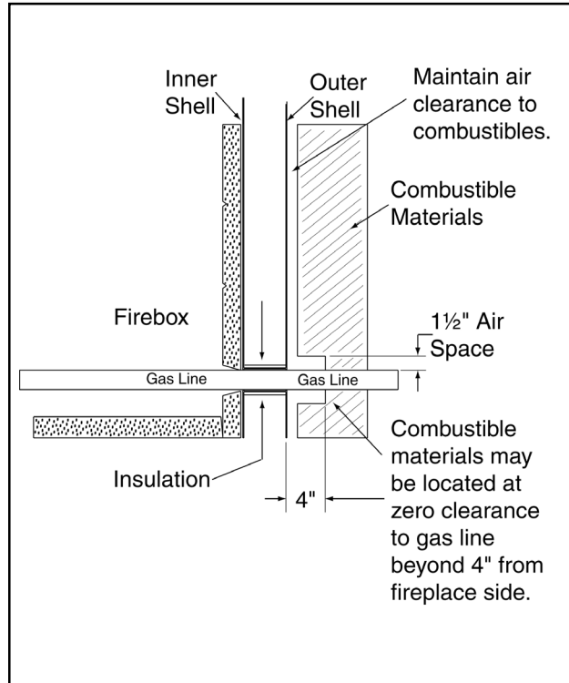
Figure 20 - Air Clearance Around Gas Line
