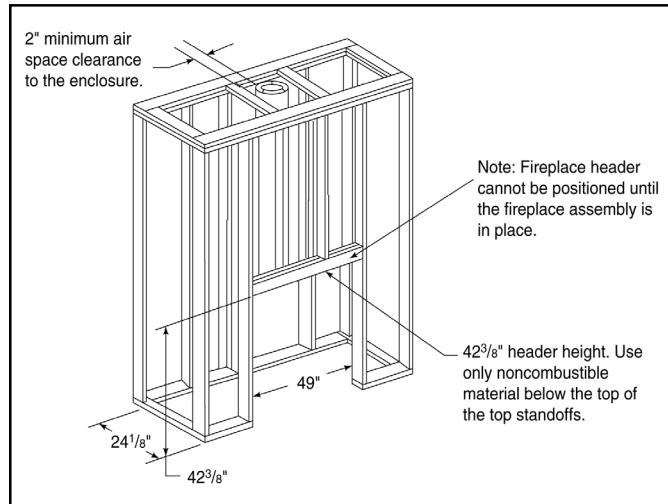
Figure 5 - Framing the Fireplace
