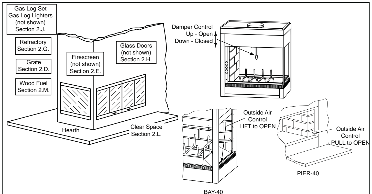
Figure 2.1 General Operating Parts
