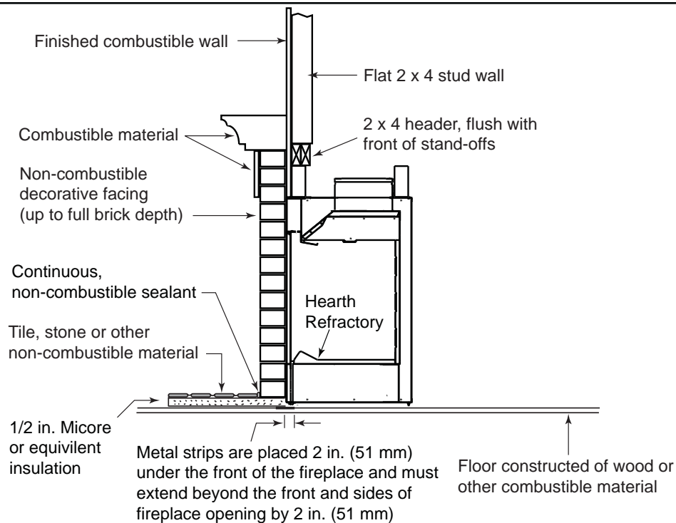
Figure 11.3 Decorative Facing
